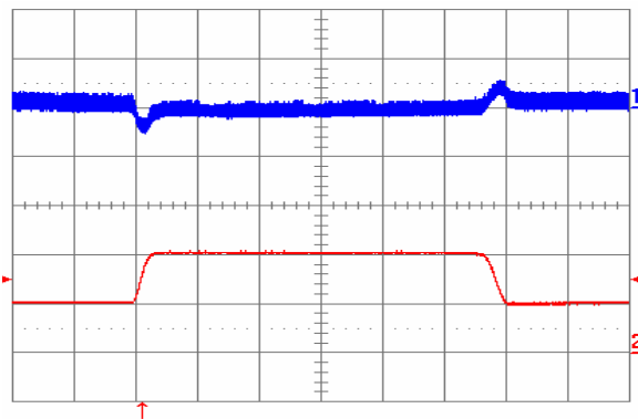
Fig. 1.2V.9: Output voltage response to load current step-change (10A - 20A - 10A) at V_{in} = 48V . Top trace: output voltage (100mV/div.). Bottom trace: load current (10A/div.). Current slew rate: 0.1A/ \mu s . C_o = 1\mu F ceramic. Time scale: 0.2ms/div.
