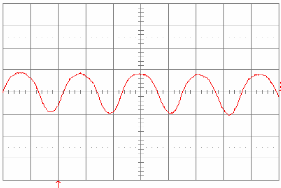
Fig. 1.8V.13: Input reflected ripple current, i_c (50mA/div.), measured at input terminals at full rated load current and V_{in} = 48\text{V} . Refer to Fig. 1.8V.12 for test setup. Time scale: 1\mu\text{s}/\text{div} .
