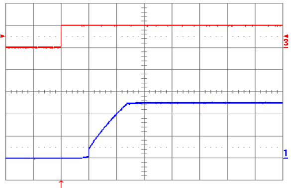
Fig. 2.5V.8: Turn-on transient at full rated load current (resistive) plus 10,000 \mu F at V_{in} = 48V , triggered via ON/OFF pin. Top trace: ON/OFF signal (5V/div.). Bottom trace: output voltage (1V/div.). Time scale: 2ms/div.
