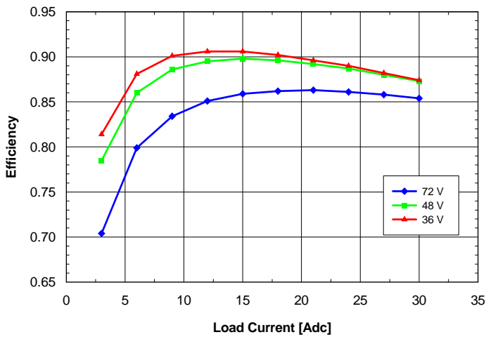
Fig. 1.8V.3: Efficiency vs. load current and input voltage for SQE48T30018 converter mounted vertically with air flowing from pin 3 to pin 1 at a rate of 300 LFM (1.5m/s) and T_a = 25^\circ\text{C} .
