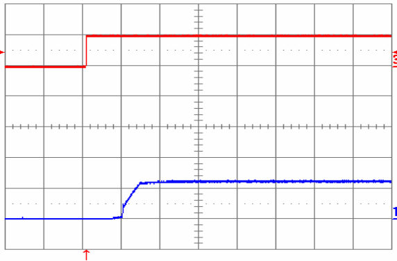
Fig. 1.2V.7: Turn-on transient at full rated load current (resistive) with no output capacitor at V_{in} = 48V , triggered via ON/OFF pin. Top trace: ON/OFF signal (5V/div.). Bottom trace: output voltage (1V/div.). Time scale: 2ms/div.
