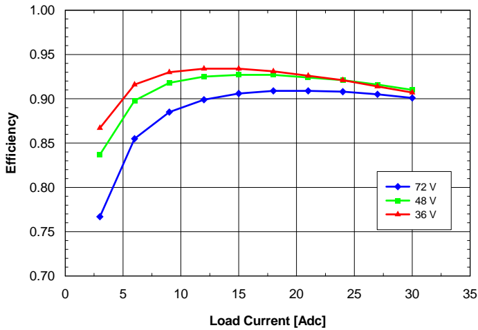
Fig. 3.3V.3: Efficiency vs. load current and input voltage for SQE48T30033 converter mounted vertically with air flowing from pin 3 to pin 1 at a rate of 300 LFM (1.5m/s) and T_a = 25^\circ\text{C} .
