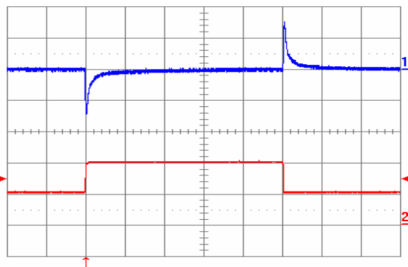
Fig. 1.8V.10: Output voltage response to load current step-change (10A – 20A – 10A) at V_{in} = 48V . Top trace: output voltage (100mV/div.). Bottom trace: load current (10A/div.). Current slew rate: 5A/ \mu s . C_o = 470\mu F POS + 1 \mu F ceramic. Time scale: 0.2ms/div.
