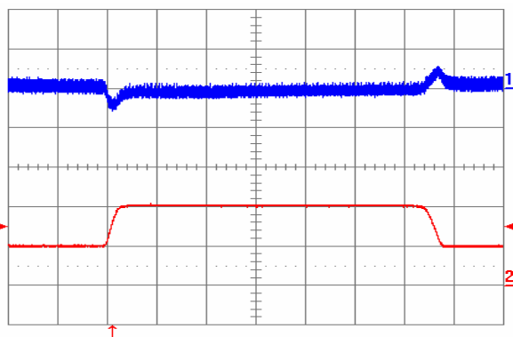
Fig. 1.5V.9: Output voltage response to load current step-change (10A – 20A – 10A) at V_{in} = 48V . Top trace: output voltage (100mV/div.). Bottom trace: load current (10A/div.). Current slew rate: 0.1A/ \mu s . C_o = 1\mu F ceramic. Time scale: 0.2ms/div.
