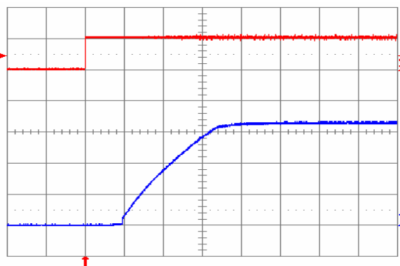
Fig. 3.3V.8: Turn-on transient at full rated load current (resistive) plus 10,000 \mu F at V_{in} = 48V , triggered via ON/OFF pin. Top trace: ON/OFF signal (5V/div.). Bottom trace: output voltage (1V/div.). Time scale: 2ms/div.
