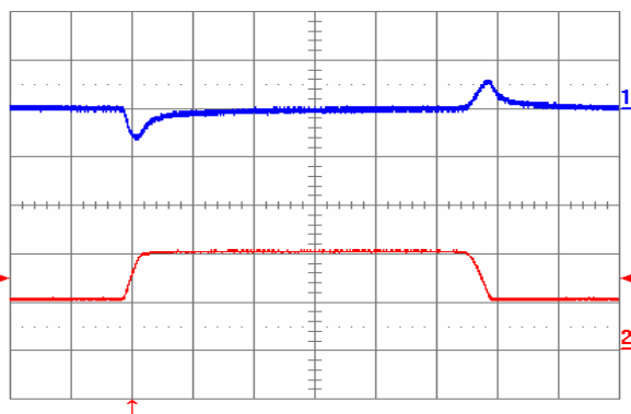
Fig. 1.8V.9: Output voltage response to load current step-change (10A – 20A – 10A) at V_{in} = 48V . Top trace: output voltage (100mV/div.). Bottom trace: load current (10A/div.). Current slew rate: 0.1A/ \mu s . C_o = 1\mu F ceramic. Time scale: 0.2ms/div.
