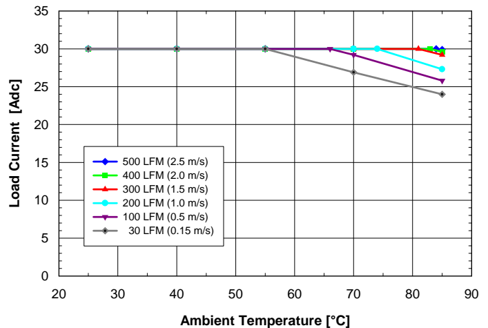
Fig. 1.2V.2: Available load current vs. ambient air temperature and airflow rates for SQE48T30012 converter with D height pins mounted horizontally with air flowing from pin 3 to pin 1, MOSFET temperature \leq 120^\circ\text{C} , V_{in} = 48\text{V} .
