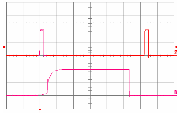
Fig. 2.5V.16: Load current (top trace, 20A/div., 20ms/div.) into a 10 mΩ short circuit during restart, at V in = 48V. Bottom trace (20A/div., 1ms/div.) is an expansion of the on-time portion of the top trace.
