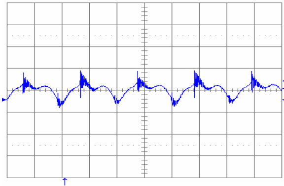
Fig. 1.2V.11: Output voltage ripple (20mV/div.) at full rated load current into a resistive load with C_o = 10\mu\text{F} tantalum + 1\mu\text{F} ceramic and V_{in} = 48\text{V} . Time scale: 1\mu\text{s}/\text{div} .
