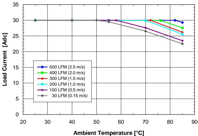
Fig. 1.8V.1: Available load current vs. ambient air temperature and airflow rates for SQE48T30018 converter with D height pins mounted vertically with air flowing from pin 3 to pin 1, MOSFET temperature \leq 120^{\circ}\text{C} , V_{in} = 48\text{ V} .
