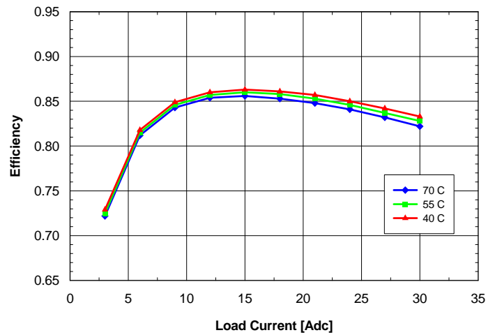
Fig. 1.2V.4: Efficiency vs. load current and ambient temperature for SQE48T30012 converter mounted vertically with V_{in} = 48\text{V} and air flowing from pin 3 to pin 1 at a rate of 200 LFM (1.0m/s).
