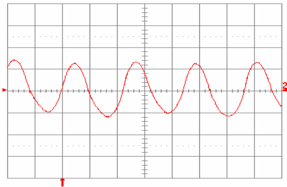
Fig. 3.3V.13: Input reflected ripple current, i_c (50mA/div.), measured at input terminals at full rated load current and V_{in} = 48\text{V} . Refer to Fig. 3.3V.12 for test setup. Time scale: 1µs/div.
