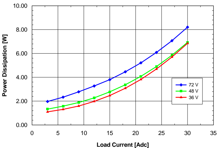
Fig. 1.2V.5: Power dissipation vs. load current and input voltage for SQE48T30012 converter mounted vertically with air flowing from pin 3 to pin 1 at a rate of 300 LFM (1.5m/s) and T_a = 25^\circ\text{C} .
