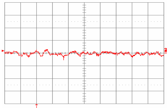
Fig. 2.5V.14: Input reflected ripple current, i_s (10mA/div.), measured through 10\mu\text{H} at the source at full rated load current and V_{in} = 48\text{V} . Refer to Fig. 2.5V.12 for test setup. Time scale: 1\mu\text{s}/\text{div} .
