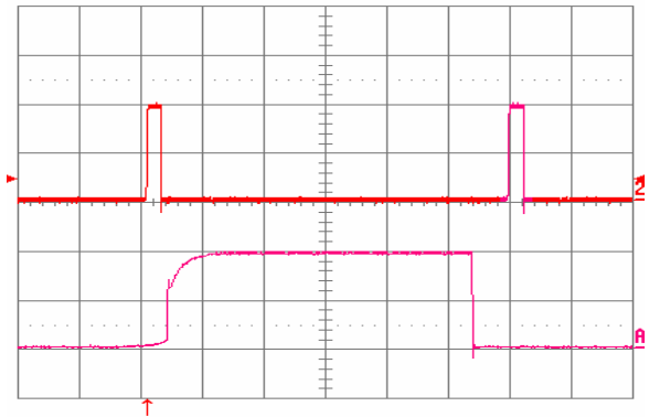
Fig. 1.2V.16: Load current (top trace, 20A/div., 20ms/div.) into a 10 mΩ short circuit during restart, at Vin = 48V. Bottom trace (20A/div., 1ms/div.) is an expansion of the on-time portion of the top trace.
