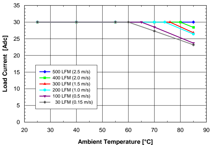
Fig. 1.5V.1: Available load current vs. ambient air temperature and airflow rates for SQE48T30015 converter with D height pins mounted vertically with air flowing from pin 3 to pin 1, MOSFET temperature \leq 120^{\circ}\text{C} , V_{in} = 48\text{V} .
