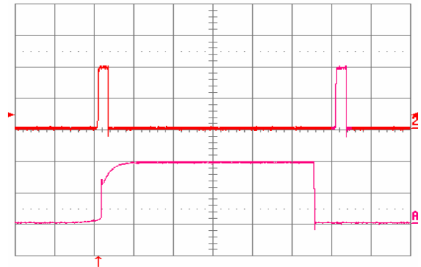
Fig. 1.8V.16: Load current (top trace, 20A/div., 20ms/div.) into a 10 mΩ short circuit during restart, at Vin = 48V. Bottom trace (20A/div., 1ms/div.) is an expansion of the on-time portion of the top trace.
