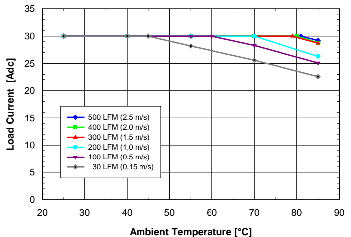
Fig. 1.5V.2: Available load current vs. ambient air temperature and airflow rates for SQE48T30015 converter with D height pins mounted horizontally with air flowing from pin 3 to pin 1, MOSFET temperature \leq 120^{\circ}\text{C} , V_{in} = 48\text{V} .
