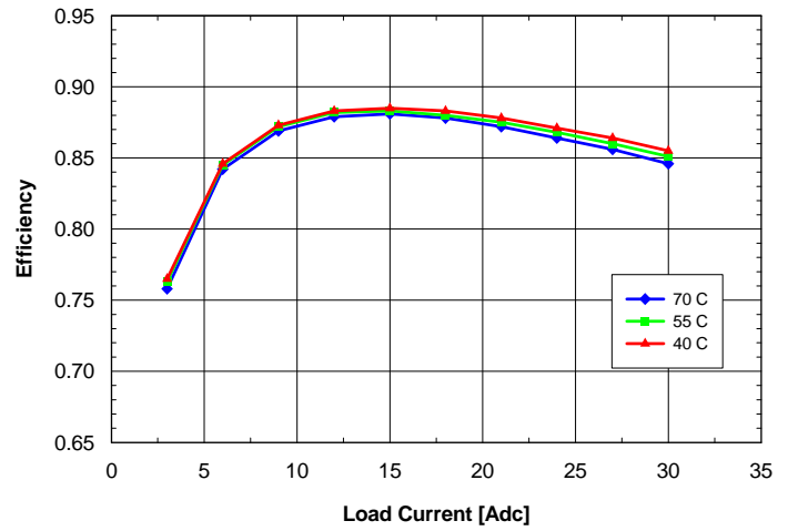
Fig. 1.5V.4: Efficiency vs. load current and ambient temperature for SQE48T30015 converter mounted vertically with V_{in} = 48\text{V} and air flowing from pin 3 to pin 1 at a rate of 200 LFM (1.0m/s).
