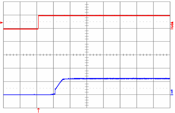
Fig. 1.2V.8: Turn-on transient at full rated load current (resistive) plus 10,000 \mu F at V_{in} = 48V , triggered via ON/OFF pin. Top trace: ON/OFF signal (5V/div.). Bottom trace: output voltage (1V/div.). Time scale: 2ms/div.
