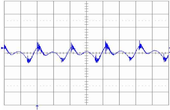
Fig. 1.5V.11: Output voltage ripple (20mV/div.) at full rated load current into a resistive load with C_o = 10\mu\text{F} tantalum + 1\mu\text{F} ceramic and V_{in} = 48\text{V} . Time scale: 1\mu\text{s}/\text{div} .
