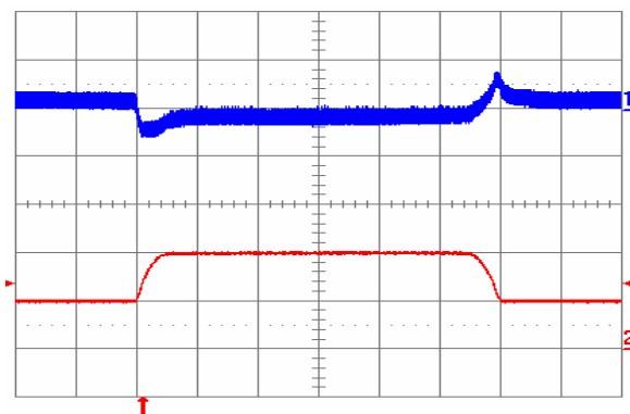
Fig. 3.3V.9: Output voltage response to load current step-change (10A – 20A – 10A) at V_{in} = 48V . Top trace: output voltage (100mV/div.). Bottom trace: load current (10A/div.). Current slew rate: 0.1A/ \mu s . C_o = 1\mu F ceramic. Time scale: 0.2ms/div.
