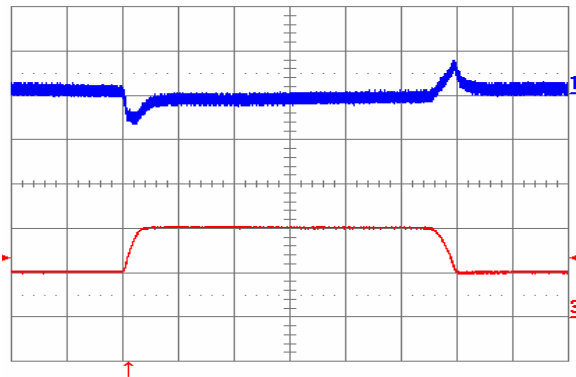
Fig. 2.5V.9: Output voltage response to load current step-change (10A – 20A – 10A) at V_{in} = 48V . Top trace: output voltage (100mV/div.). Bottom trace: load current (10A/div.). Current slew rate: 0.1A/ \mu s . C_o = 1\mu F ceramic. Time scale: 0.2ms/div.
