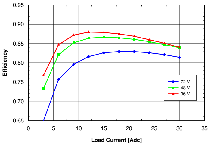
Fig. 1.2V.3: Efficiency vs. load current and input voltage for SQE48T30012 converter mounted vertically with air flowing from pin 3 to pin 1 at a rate of 300 LFM (1.5m/s) and T_a = 25^\circ\text{C} .
