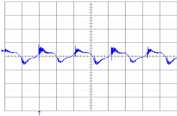
Fig. 2.5V.11: Output voltage ripple (20mV/div.) at full rated load current into a resistive load with C_o = 10\mu\text{F} tantalum + 1\mu\text{F} ceramic and V_{in} = 48\text{V} . Time scale: 1\mu\text{s}/\text{div} .
