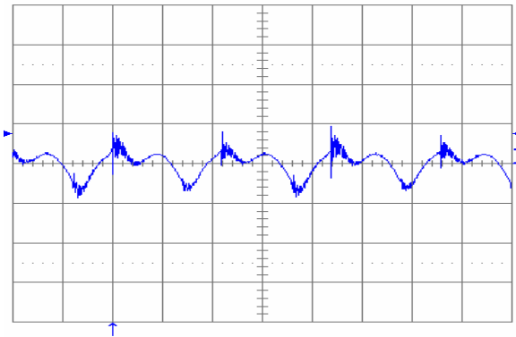
Fig. 1.8V.11: Output voltage ripple (20mV/div.) at full rated load current into a resistive load with C_o = 10\mu\text{F} tantalum + 1\mu\text{F} ceramic and V_{in} = 48\text{V} . Time scale: 1\mu\text{s}/\text{div} .
