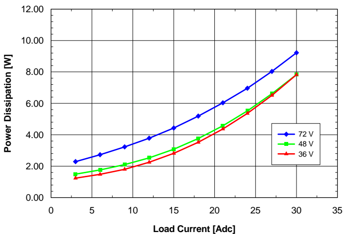
Fig. 1.8V.5: Power dissipation vs. load current and input voltage for SQE48T30018 converter mounted vertically with air flowing from pin 3 to pin 1 at a rate of 300 LFM (1.5m/s) and T_a = 25^\circ\text{C} .
