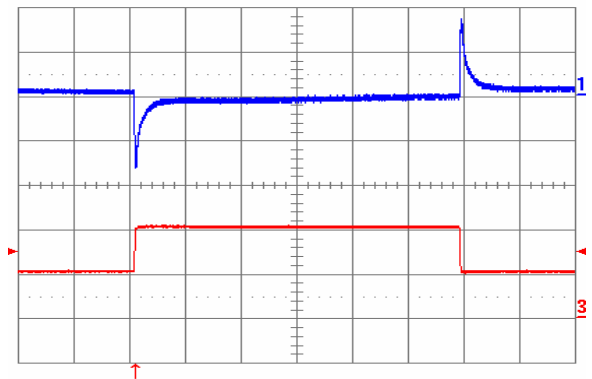
Fig. 2.5V.10: Output voltage response to load current step-change (10A – 20A – 10A) at V_{in} = 48V . Top trace: output voltage (100mV/div.). Bottom trace: load current (10A/div.). Current slew rate: 5A/ \mu s . C_o = 470\mu F POS + 1 \mu F ceramic. Time scale: 0.2ms/div.
