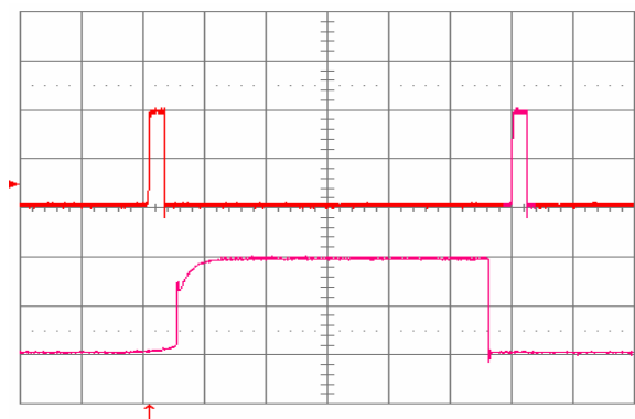
Fig. 1.5V.16: Load current (top trace, 20A/div., 20ms/div.) into a 10 mΩ short circuit during restart, at Vin = 48V. Bottom trace (20A/div., 1ms/div.) is an expansion of the on-time portion of the top trace.
