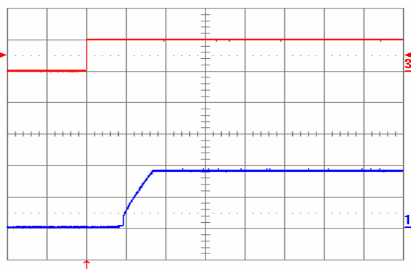
Fig. 1.8V.8: Turn-on transient at full rated load current (resistive) plus 10,000 \mu F at V_{in} = 48V , triggered via ON/OFF pin. Top trace: ON/OFF signal (5V/div.). Bottom trace: output voltage (1V/div.). Time scale: 2ms/div.
