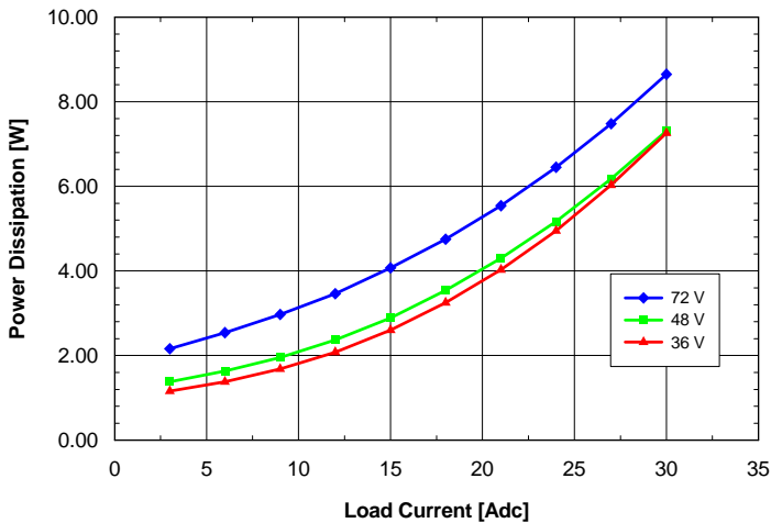
Fig. 1.5V.5: Power dissipation vs. load current and input voltage for SQE48T30015 converter mounted vertically with air flowing from pin 3 to pin 1 at a rate of 300 LFM (1.5m/s) and T_a = 25^\circ\text{C} .
