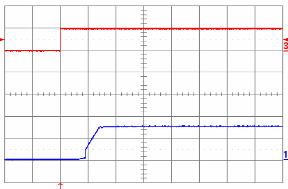
Fig. 1.5V.7: Turn-on transient at full rated load current (resistive) with no output capacitor at V_{in} = 48V , triggered via ON/OFF pin. Top trace: ON/OFF signal (5V/div.). Bottom trace: output voltage (1V/div.). Time scale: 2ms/div.
