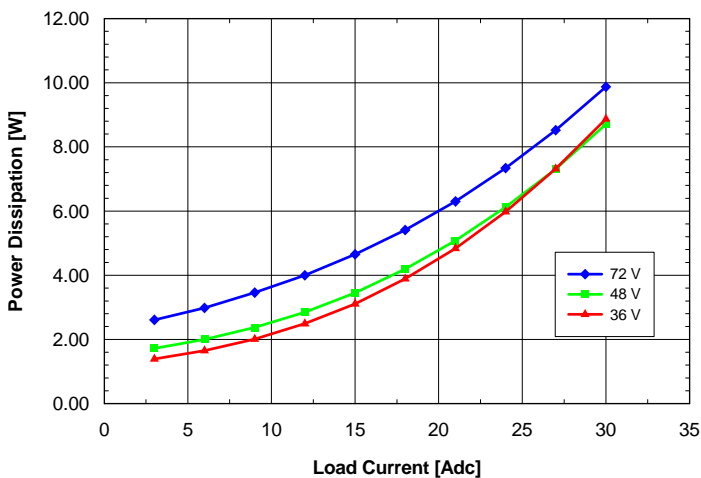
Fig. 2.5V.5: Power dissipation vs. load current and input voltage for SQE48T30025 converter mounted vertically with air flowing from pin 3 to pin 1 at a rate of 300 LFM (1.5m/s) and T_a = 25^\circ\text{C} .
