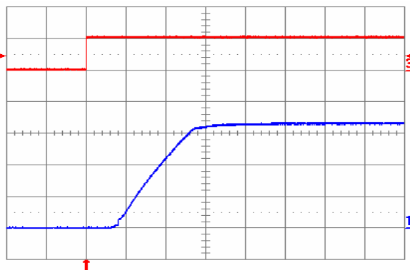
Fig. 3.3V.7: Turn-on transient at full rated load current (resistive) with no output capacitor at V_{in} = 48V , triggered via ON/OFF pin. Top trace: ON/OFF signal (5V/div.). Bottom trace: output voltage (1V/div.). Time scale: 2ms/div.
