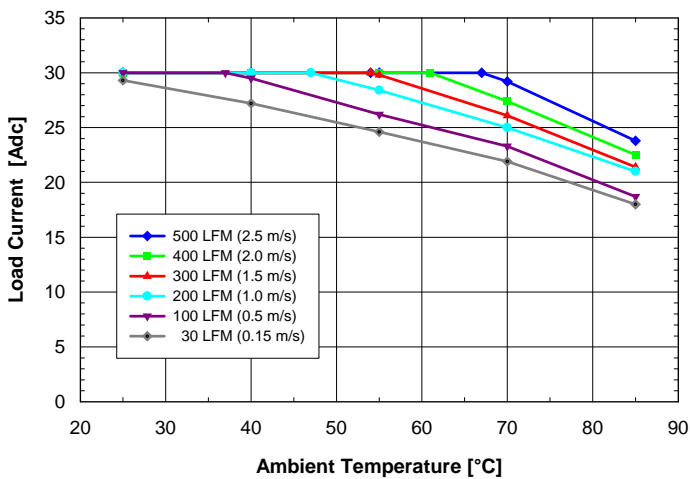
Fig. 3.3V.1: Available load current vs. ambient air temperature and airflow rates for SQE48T30033 converter with D height pins mounted vertically with air flowing from pin 3 to pin 1, MOSFET temperature \leq 120^\circ\text{C} , V_{in} = 48\text{V} .
