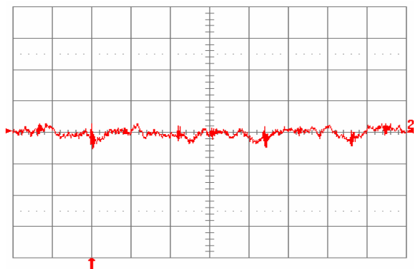
Fig. 3.3V.14: Input reflected ripple current, i_s (10mA/div.), measured through 10µH at the source at full rated load current and V_{in} = 48\text{V} . Refer to Fig. 3.3V.12 for test setup. Time scale: 1µs/div.
