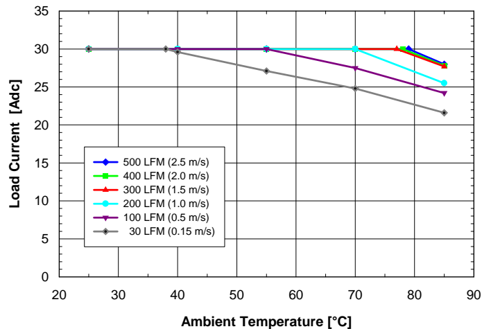
Fig. 1.8V.2: Available load current vs. ambient air temperature and airflow rates for SQE48T30018 converter with D height pins mounted horizontally with air flowing from pin 3 to pin 1, MOSFET temperature \leq 120^{\circ}\text{C} , V_{in} = 48\text{ V} .
