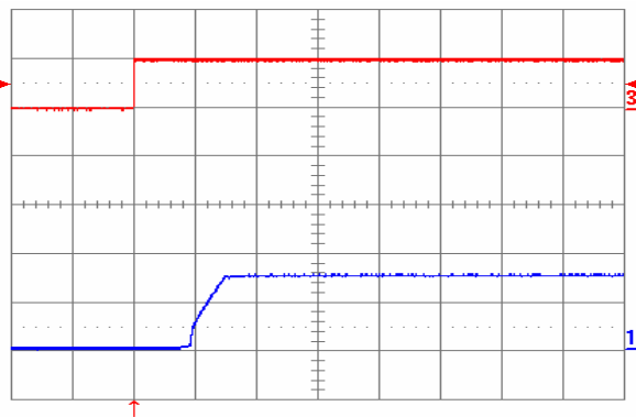
Fig. 1.5V.8: Turn-on transient at full rated load current (resistive) plus 10,000 \mu F at V_{in} = 48V , triggered via ON/OFF pin. Top trace: ON/OFF signal (5V/div.). Bottom trace: output voltage (1V/div.). Time scale: 2ms/div.
