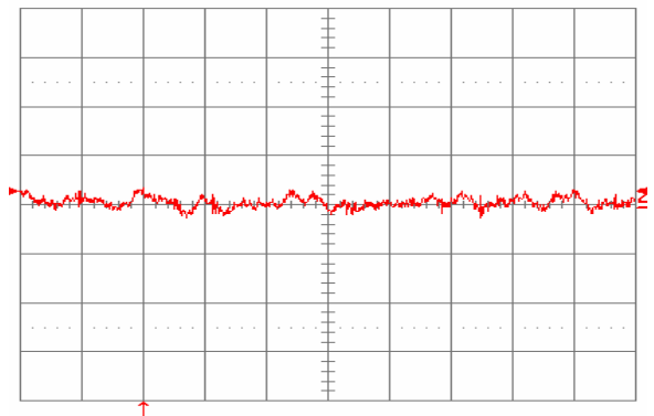
Fig. 1.5V.14: Input reflected ripple current, i_s (10mA/div.), measured through 10\mu\text{H} at the source at full rated load current and V_{in} = 48\text{V} . Refer to Fig 1.5V.12 for test setup. Time scale: 1\mu\text{s}/\text{div} .
