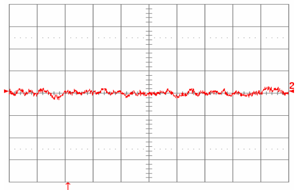
Fig. 1.2V.14: Input reflected ripple current, i_s (10mA/div.), measured through 10\mu\text{H} at the source at full rated load current and V_{in} = 48\text{V} . Refer to Fig. 1.2V.12 for test setup. Time scale: 1\mu\text{s}/\text{div} .
