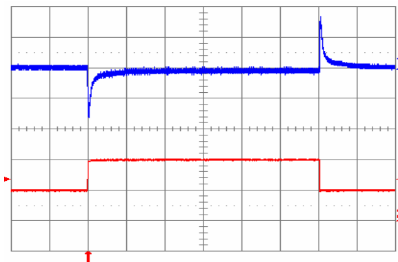
Fig. 3.3V.10: Output voltage response to load current step-change (10A – 20A – 10A) at V_{in} = 48V . Top trace: output voltage (100mV/div.). Bottom trace: load current (10A/div.). Current slew rate: 5A/ \mu s . C_o = 470\mu F POS + 1 \mu F ceramic. Time scale: 0.2ms/div.
