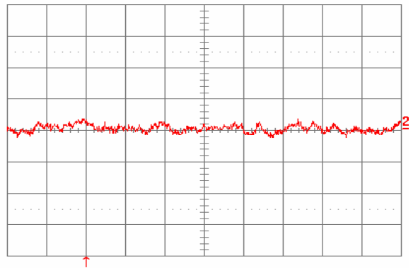
Fig. 1.8V.14: Input reflected ripple current, i_s (10mA/div.), measured through 10\mu\text{H} at the source at full rated load current and V_{in} = 48\text{V} . Refer to Fig. 1.8V.12 for test setup. Time scale: 1\mu\text{s}/\text{div} .
