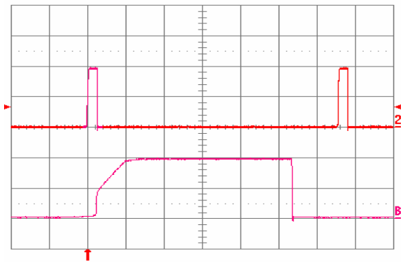
Fig. 3.3V.16: Load current (top trace, 20A/div., 20ms/div.) into a 10mΩ short circuit during restart, at Vin = 48V. Bottom trace (20A/div., 1ms/div.) is an expansion of the on-time portion of the top trace.
