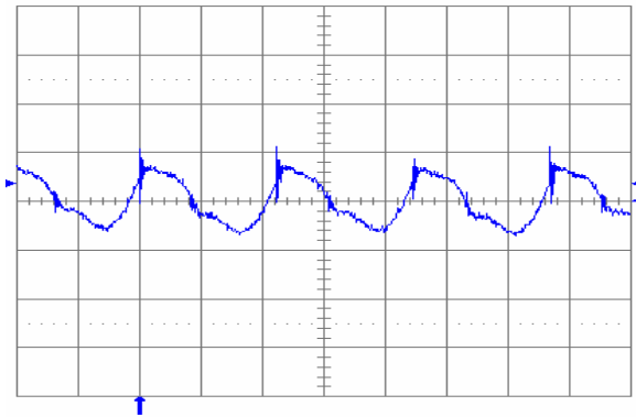
Fig. 3.3V.11: Output voltage ripple (20mV/div.) at full rated load current into a resistive load with C_o = 10\mu\text{F} tantalum + 1µF ceramic and V_{in} = 48\text{V} . Time scale: 1µs/div.
