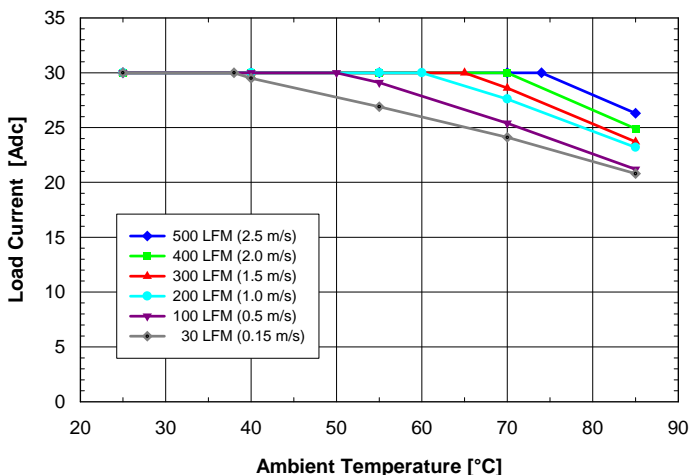
Fig. 2.5V.1: Available load current vs. ambient air temperature and airflow rates for SQE48T30025 converter with D height pins mounted vertically with air flowing from pin 3 to pin 1, MOSFET temperature \leq 120^\circ\text{C} , V_{in} = 48\text{V} .
