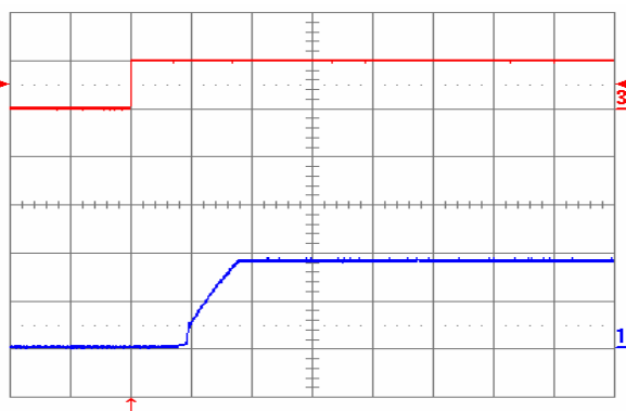
Fig. 1.8V.7: Turn-on transient at full rated load current (resistive) with no output capacitor at V_{in} = 48V , triggered via ON/OFF pin. Top trace: ON/OFF signal (5V/div.). Bottom trace: output voltage (1V/div.). Time scale: 2ms/div.
