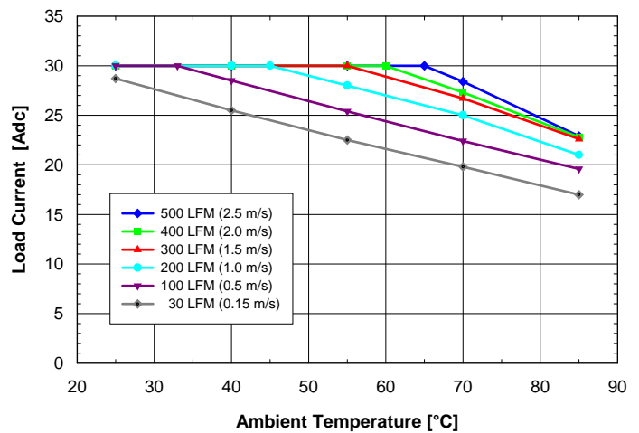
Fig. 3.3V.2: Available load current vs. ambient air temperature and airflow rates for SQE48T30033 converter with D height pins mounted horizontally with air flowing from pin 3 to pin 1, MOSFET temperature \leq 120^\circ\text{C} , V_{in} = 48\text{V} .
