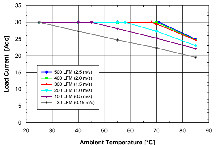
Fig. 2.5V.2: Available load current vs. ambient air temperature and airflow rates for SQE48T30025 converter with D height pins mounted horizontally with air flowing from pin 3 to pin 1, MOSFET temperature \leq 120^\circ\text{C} , V_{in} = 48\text{V} .
