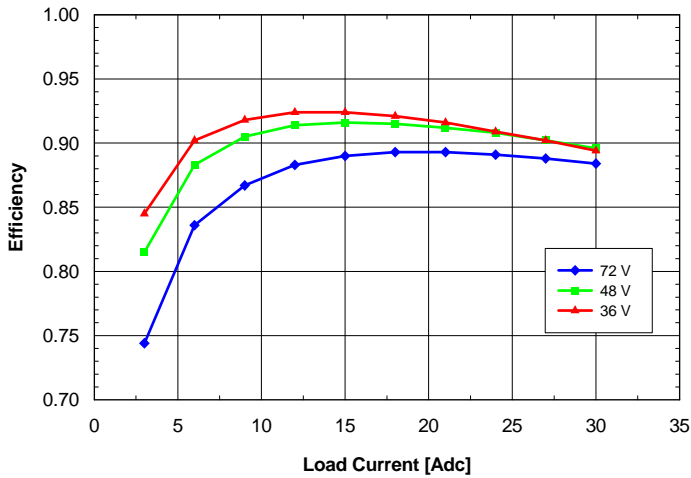
Fig. 2.5V.3: Efficiency vs. load current and input voltage for SQE48T30025 converter mounted vertically with air flowing from pin 3 to pin 1 at a rate of 300 LFM (1.5m/s) and T_a = 25^\circ\text{C} .
