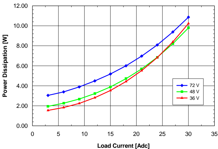
Fig. 3.3V.5: Power dissipation vs. load current and input voltage for SQE48T30033 converter mounted vertically with air flowing from pin 3 to pin 1 at a rate of 300 LFM (1.5m/s) and T_a = 25^\circ\text{C} .
