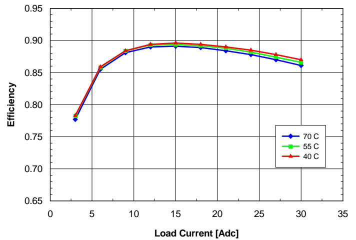
Fig. 1.8V.4: Efficiency vs. load current and ambient temperature for SQE48T30018 converter mounted vertically with V_{in} = 48\text{V} and air flowing from pin 3 to pin 1 at a rate of 200 LFM (1.0m/s).
