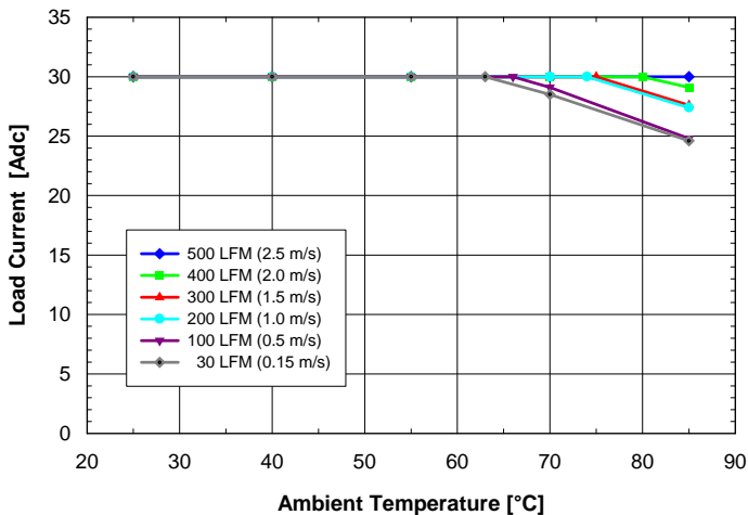
Fig. 1.2V.1: Available load current vs. ambient air temperature and airflow rates for SQE48T30012 converter with D height pins mounted vertically with air flowing from pin 3 to pin 1, MOSFET temperature \leq 120^\circ\text{C} , V_{in} = 48\text{V} .
