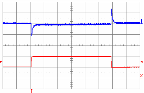
Fig. 1.2V.10: Output voltage response to load current step-change (10A - 20A - 10A) at V_{in} = 48V . Top trace: output voltage (100mV/div.). Bottom trace: load current (10A/div.). Current slew rate: 5A/ \mu s . C_o = 470\mu F POS + 1 \mu F ceramic. Time scale: 0.2ms/div.
