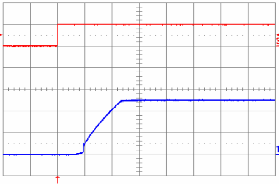
Fig. 2.5V.7: Turn-on transient at full rated load current (resistive) with no output capacitor at V_{in} = 48V , triggered via ON/OFF pin. Top trace: ON/OFF signal (5V/div.). Bottom trace: output voltage (1V/div.). Time scale: 2ms/div.
