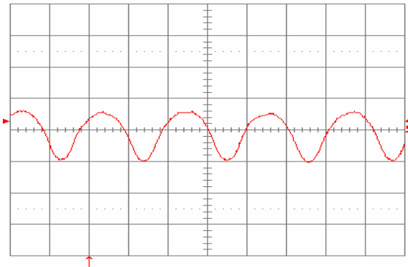
Fig. 1.5V.13: Input reflected ripple current, i_c (50mA/div.), measured at input terminals at full rated load current and V_{in} = 48\text{V} . Refer to Fig. 1.5V.12 for test setup. Time scale: 1\mu\text{s}/\text{div} .
