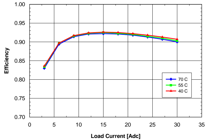
Fig. 3.3V.4: Efficiency vs. load current and ambient temperature for SQE48T30033 converter mounted vertically with V_{in} = 48\text{V} and air flowing from pin 3 to pin 1 at a rate of 200 LFM (1.0m/s).
