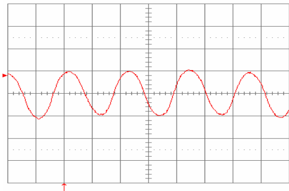
Fig. 2.5V.13: Input reflected ripple current, i_c (50 mA/div.), measured at input terminals at full rated load current and V_{in} = 48\text{V} . Refer to Fig. 2.5V.12 for test setup. Time scale: 1\mu\text{s}/\text{div} .
