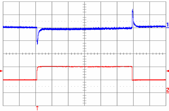
Fig. 1.5V.10: Output voltage response to load current step-change (10A – 20A – 10A) at V_{in} = 48V . Top trace: output voltage (100mV/div.). Bottom trace: load current (10A/div.). Current slew rate: 5A/ \mu s . C_o = 470\mu F POS + 1 \mu F ceramic. Time scale: 0.2ms/div.
