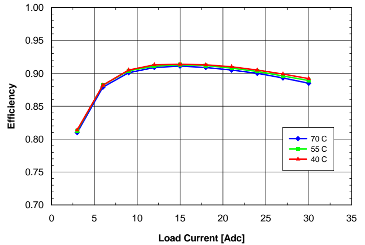
Fig. 2.5V.4: Efficiency vs. load current and ambient temperature for SQE48T30025 converter mounted vertically with V_{in} = 48\text{V} and air flowing from pin 3 to pin 1 at a rate of 200 LFM (1.0m/s).
