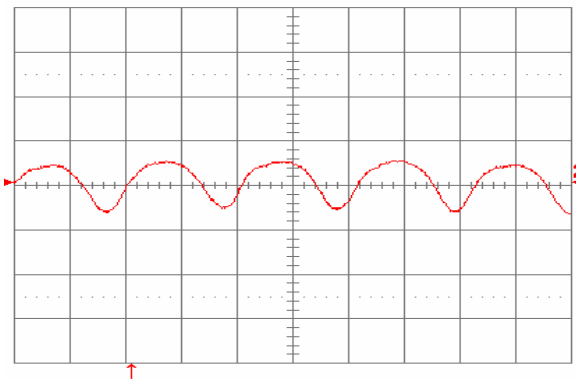
Fig. 1.2V.13: Input reflected ripple current, i_c (50 mA/div.), measured at input terminals at full rated load current and V_{in} = 48\text{V} . Refer to Fig. 1.2V.12 for test setup. Time scale: 1\mu\text{s}/\text{div} .
