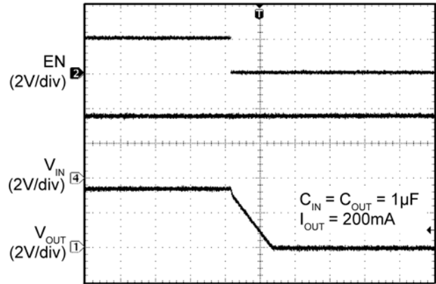
Enable Turn-Off
