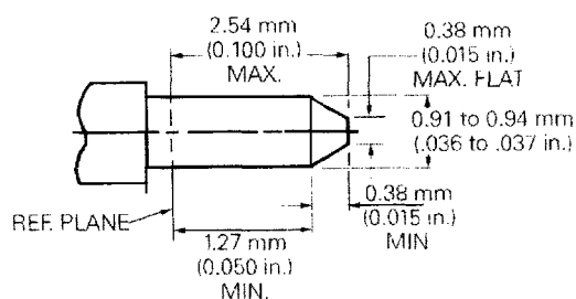
DETAIL A-1
