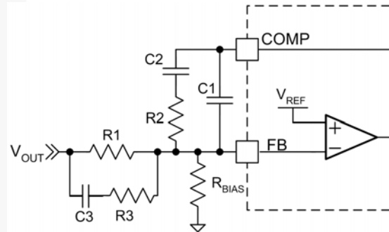
Figure 34. Compensation Network
