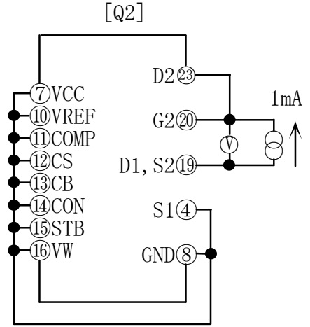
Fig.2 VGS(th)
