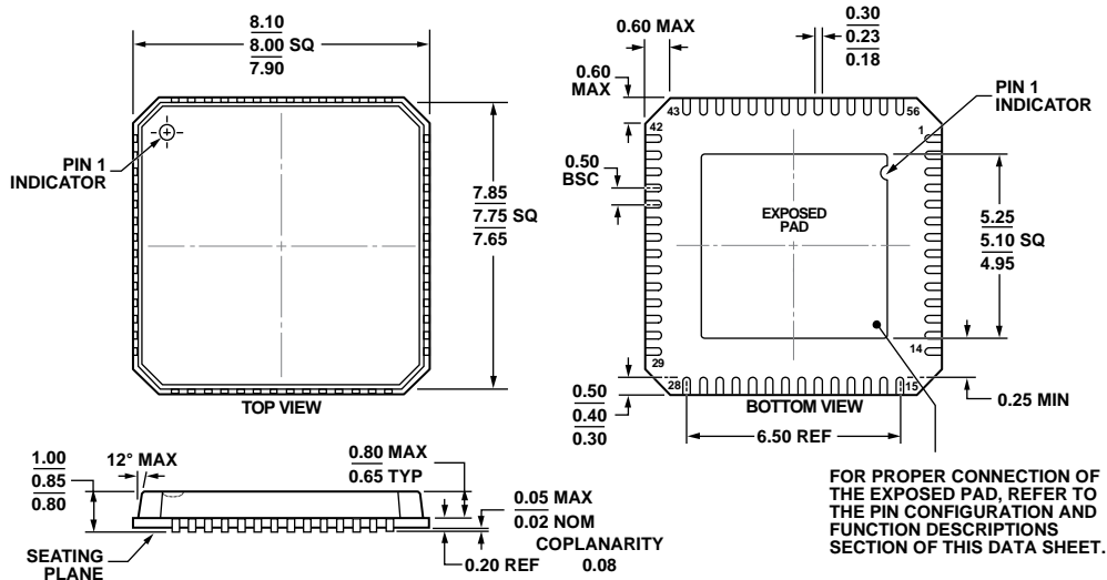
Figure 76. 56-Lead Lead Frame Chip Scale Package [LFCSP_VQ] 8 mm × 8 mm Body, Very Thin Quad (CP-56-5)
