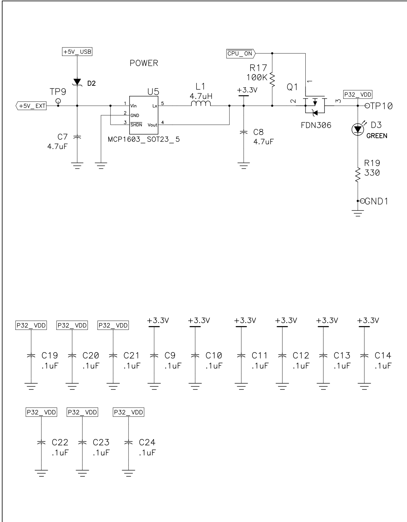
FIGURE A-6: PIC32MX SCHEMATIC, SHEET 6 OF 6 (POWER SUPPLY)
