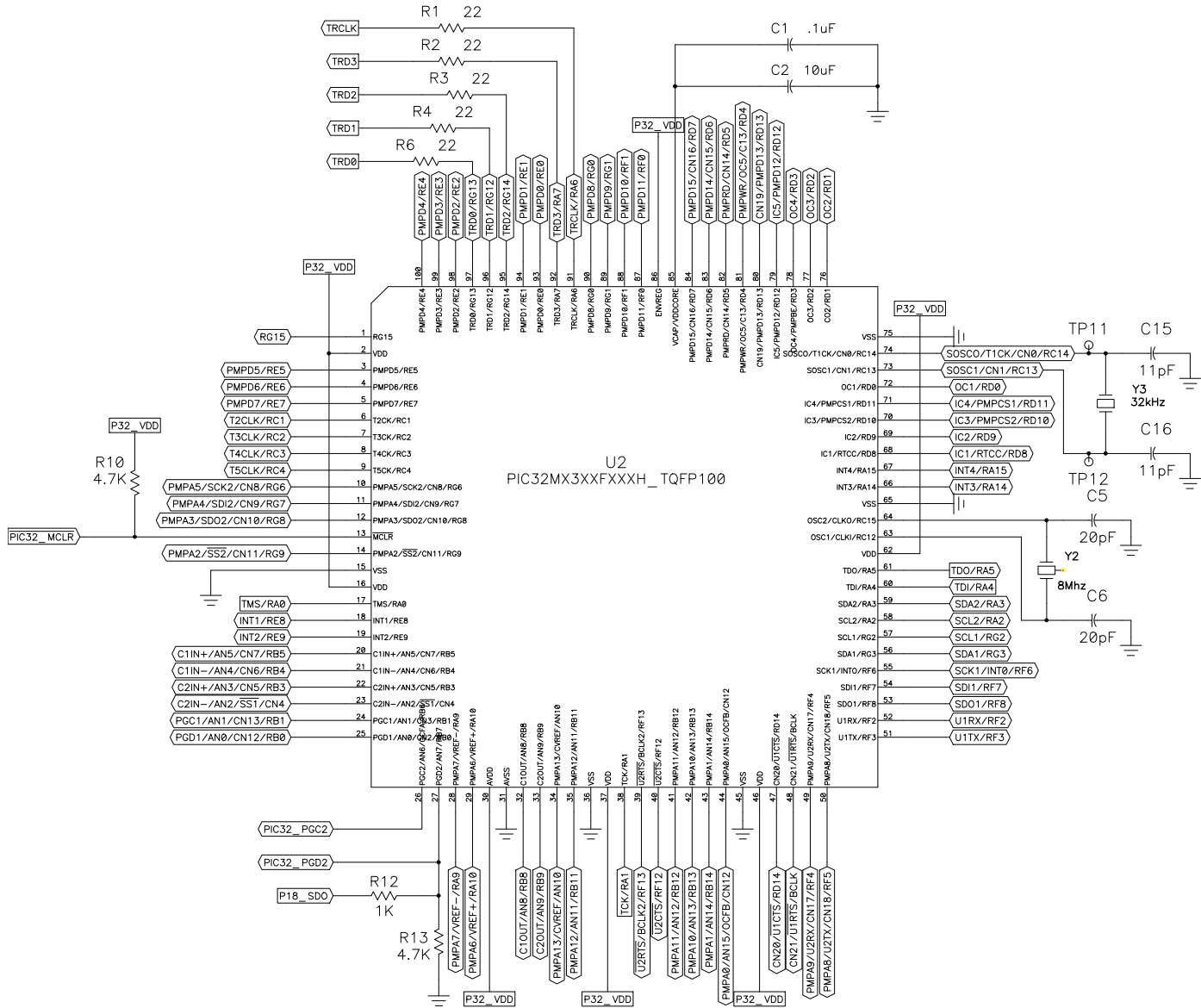
FIGURE A-2: PIC32MX SCHEMATIC, SHEET 1 OF 6 (PIC32MX CPU)
