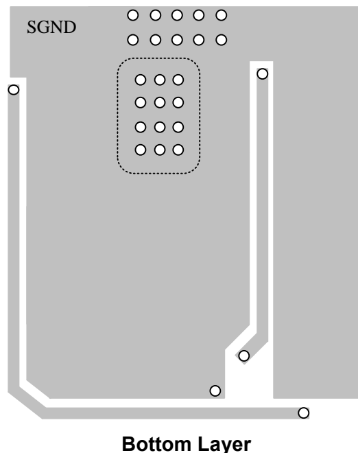
Figure 3—PCB Layout
