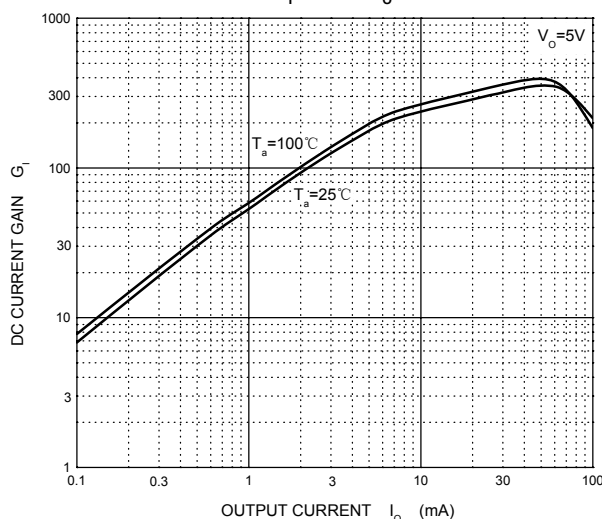
G_1 — I_O
