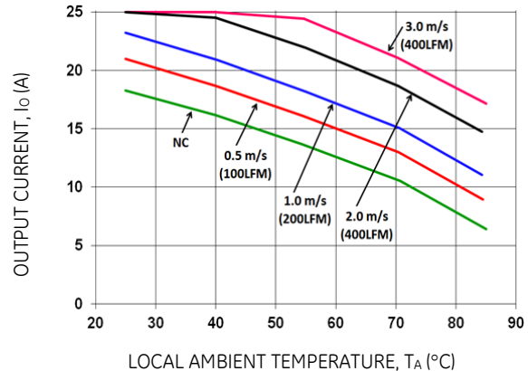
Figure 21. Output Current Derating for the Base plate EBDW025A0B-H in the Transverse Orientation; Airflow Direction from Vin(+) to Vin(-); Vin = 48V.
