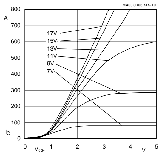
Fig. 10 Typ. output characteristic, t_p = 250 \mu s ; 125 \text{ }^\circ\text{C}
