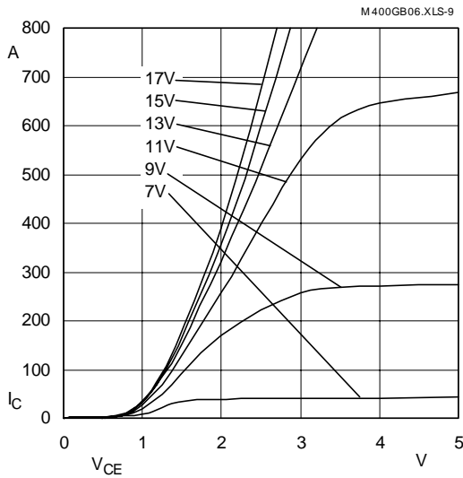
Fig. 9 Typ. output characteristic, t_p = 250 \mu s ; 25 \text{ }^\circ\text{C}
