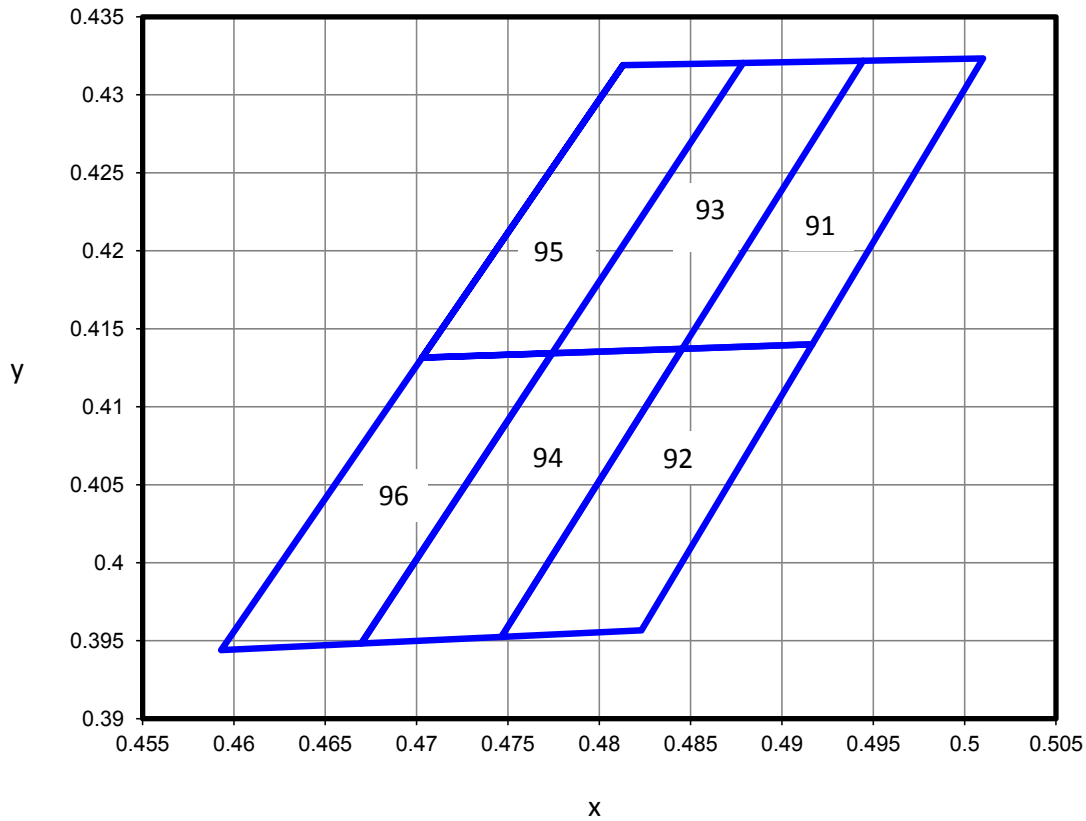
Figure 13. 2500K 1/6th color bin structure.
