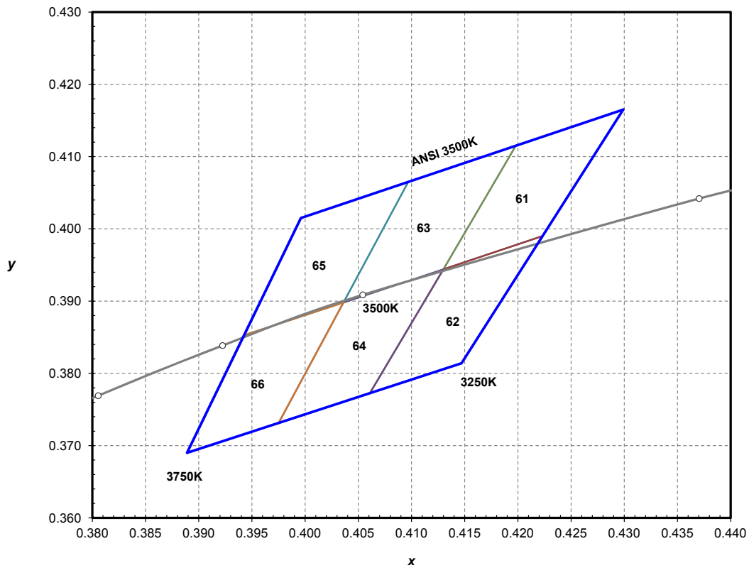
Figure 16. ANSI 3500K I/6th color bin structure.
