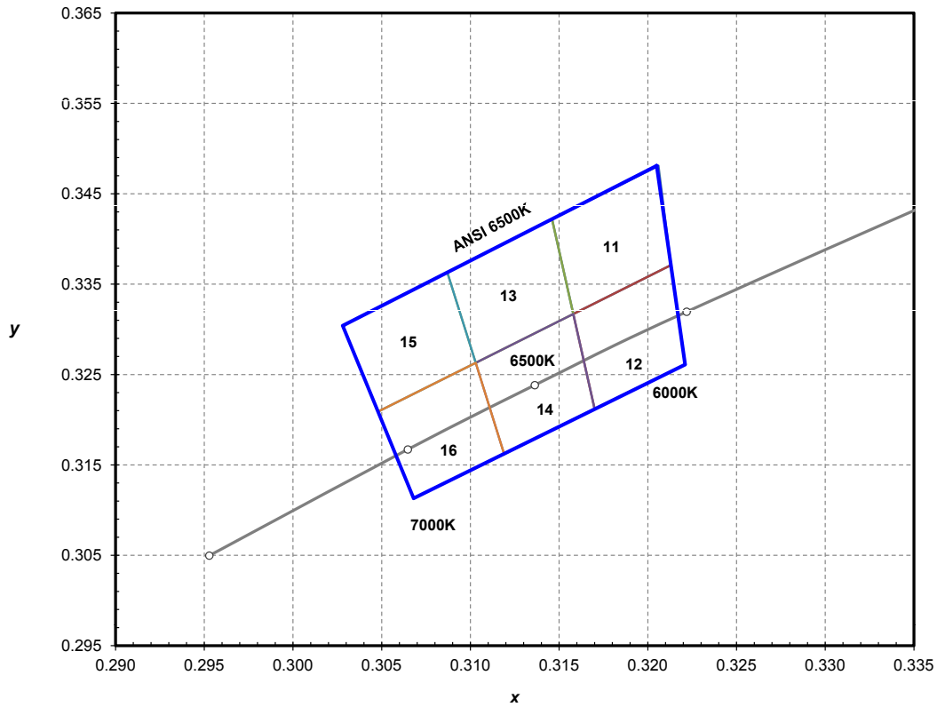
Figure 20. ANSI 6500K I/6th color bin structure.
