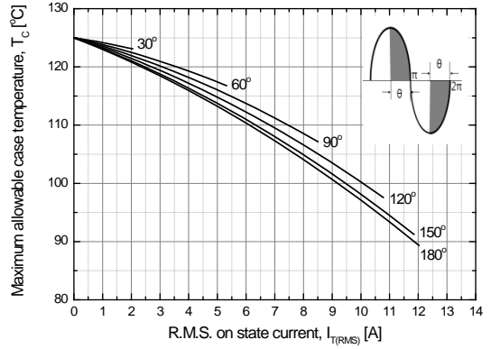
Fig 2. R.M.S. current vs. Case temperature
