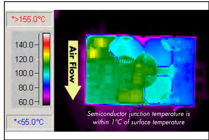
Figure 8: Thermal plot of converter at 4.4 amp load current (66W) with 55°C air flowing at the rate of 200 LFM. Air is flowing across the converter from pin 1 to pin 3 (nominal input voltage).
