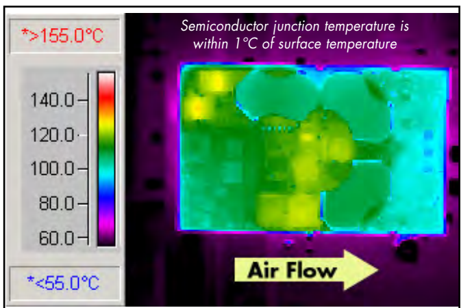
Figure 6: Thermal plot of converter at 4.5 amp load current (68W) with 55°C air flowing at the rate of 200 LFM. Air is flowing across the converter from input to output (nominal input voltage).
