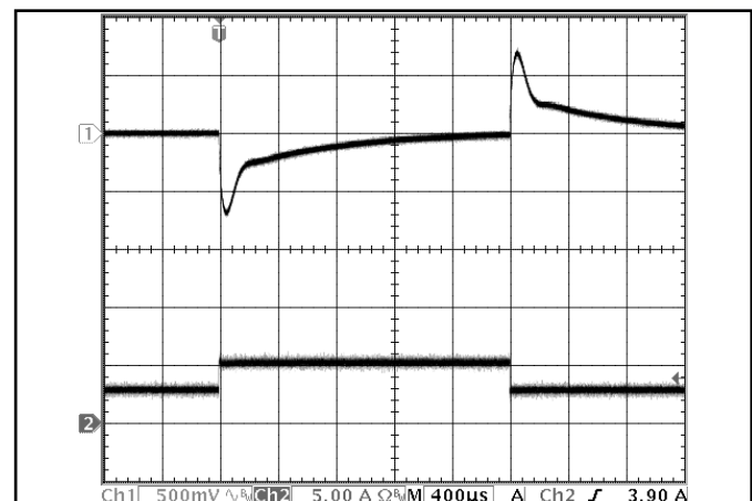
Figure 12: Output voltage response to step-change in load current (50%-75%-50% of I out (max); dI/dt = 5A/μs). Load cap: 470μF, 30 mΩ ESR tantalum capacitor and 1μF ceramic cap. Ch 1: V out (500mV/div), Ch 2: I out (5A/div).
