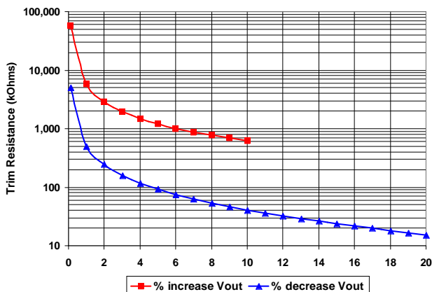
Figure C: Trim Graph for 15V out module
