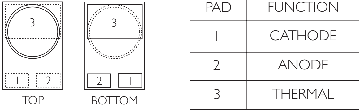
Figure 2. Pad configuration.
