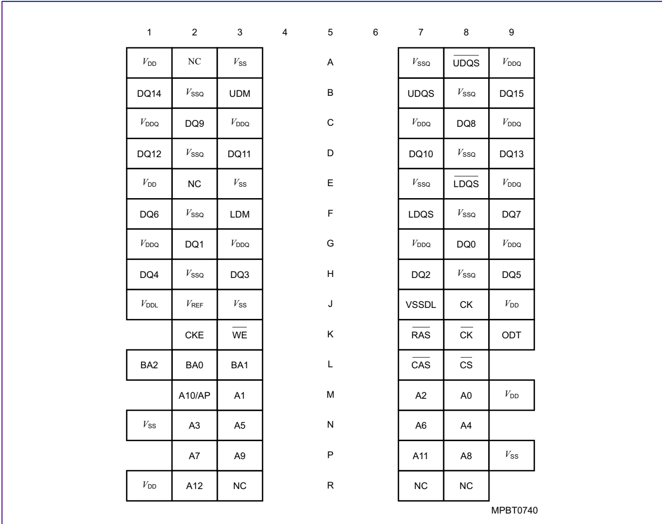
FIGURE 3 Chip Configuration for x16 Components in TFBGA-84 (Top view)
