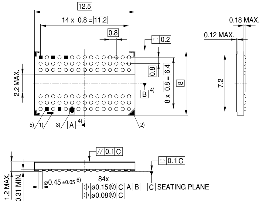
FIGURE 13 Package Outline P-TFBGA-84
