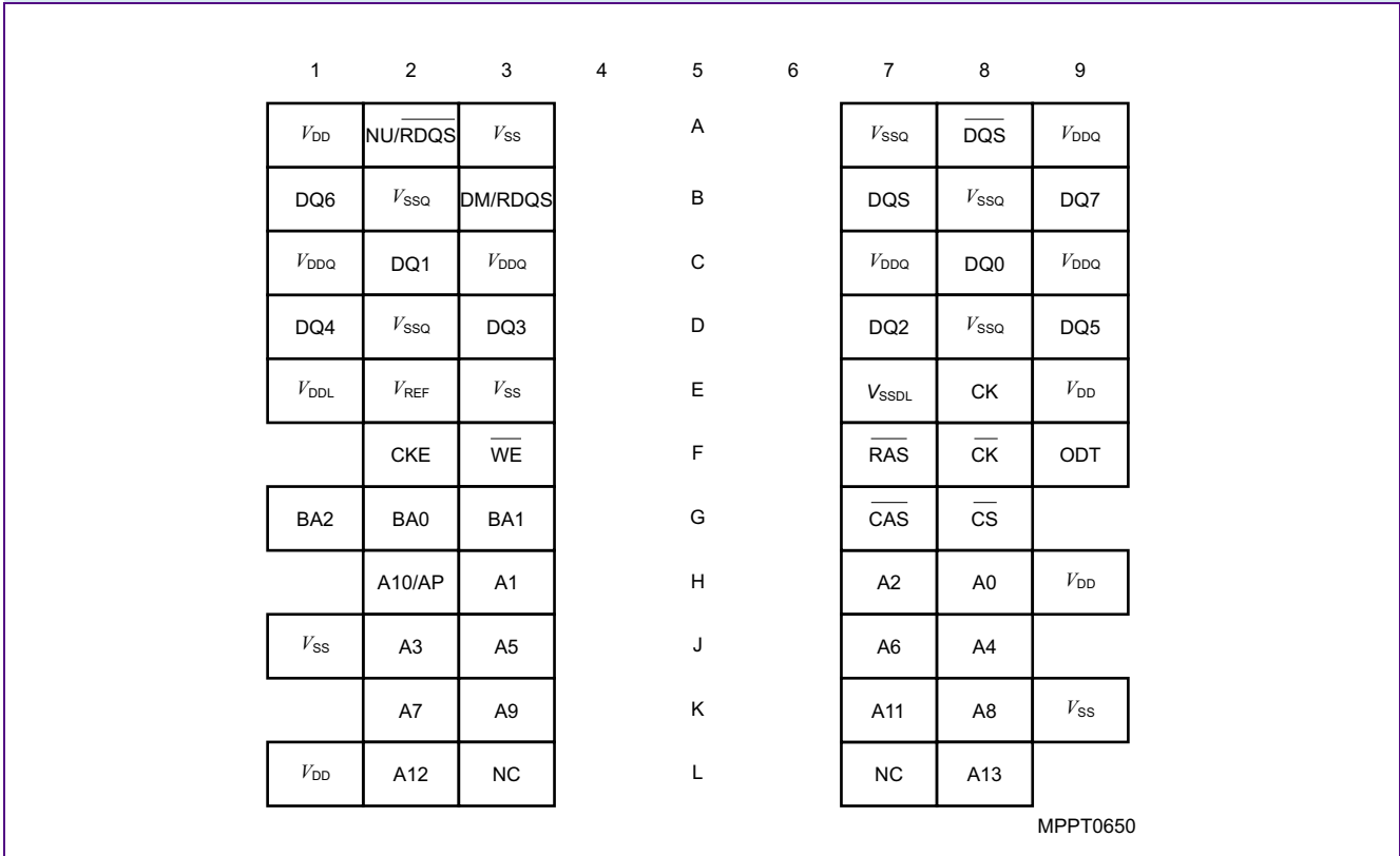
FIGURE 2 Chip Configuration for ×8 Components, TFBGA-60 (top view)
