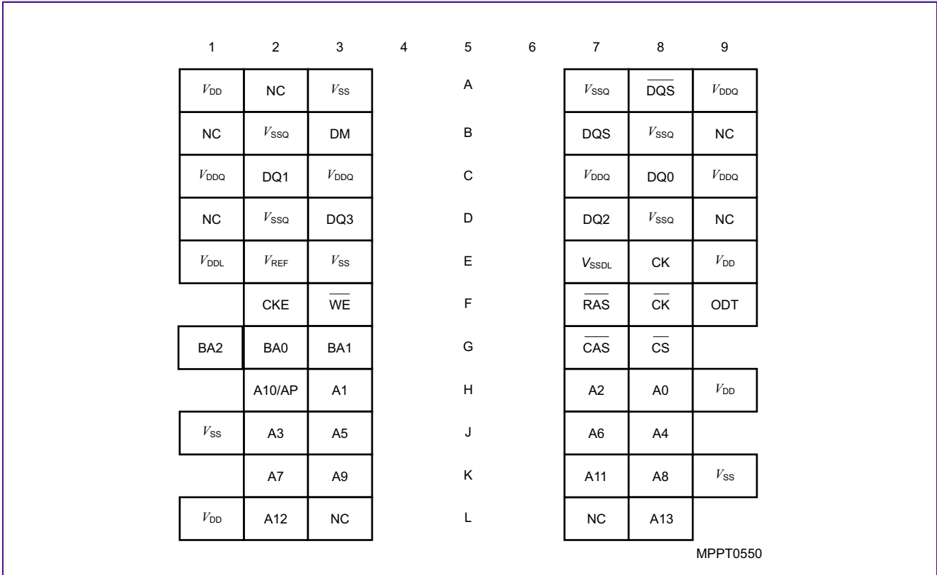
FIGURE 1 Chip Configuration for ×4 components, TFBGA-60 (top view)
