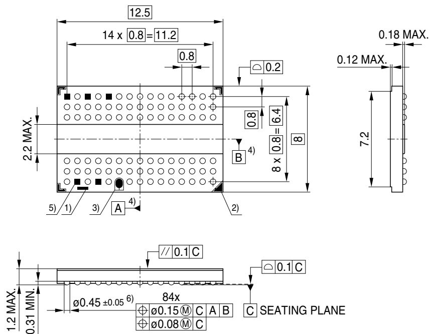
FIGURE 14 Package Outline PG-TFBGA-84
