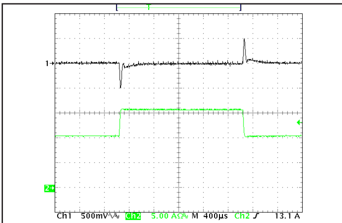
Figure 5: Output voltage response to step-change in load current (50%-75%-50% of I out (max); di/dt = 0.1A/µs. Load cap: 15µF tantalum cap and 1µF ceramic cap. Ch 1: V out , Ch 2: I out (5 A/div).
