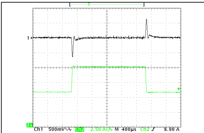
Figure 5: Output voltage response to step-change in load current (50%-75%-50% of Iout(max)); di/dt = 0.1A/\mu s . Load cap: 15μF tantalum cap and 1μF ceramic cap. Ch 1: Vout, Ch 2: Iout (2.5 A/div).
