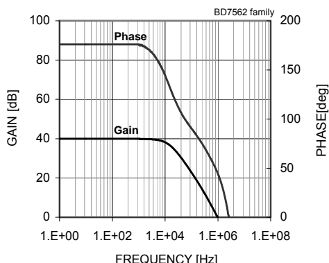
Fig.23 Gain - Frequency
