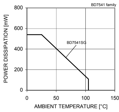
Fig.2 Derating Curve
