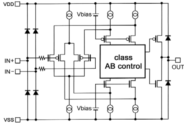
Fig1. Schematic diagram
