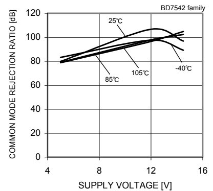
Fig. 18 Common Mode Rejection Ratio – Supply Voltage ( V_{DD}=12[V] )
