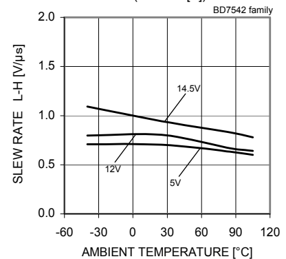
Fig. 21 Slew Rate L-H – Ambient Temperature
