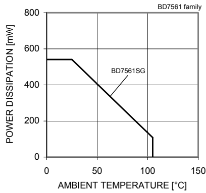
Fig.2 Derating Curve
