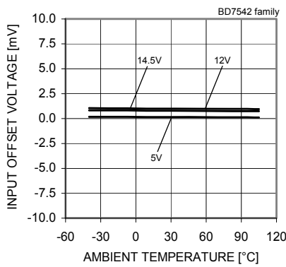
Fig. 14 Input Offset Voltage – Ambient Temperature ( V_{icm}=V_{DD} , V_{OUT}=V_{DD}/2 )
