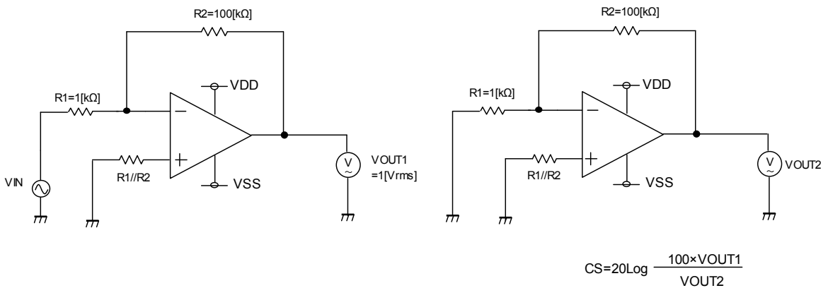
Fig5. Test circuit3
