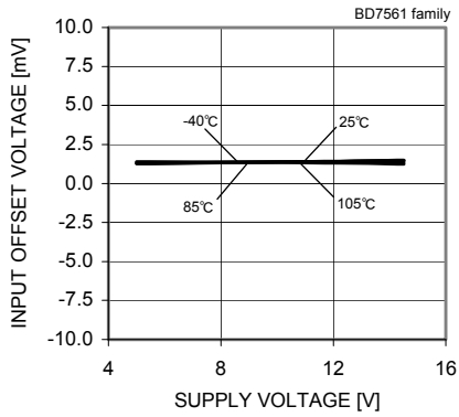
Fig.13 Input Offset Voltage – Supply Voltage ( V_{icm}=V_{DD} , V_{OUT}=V_{DD}/2 )
