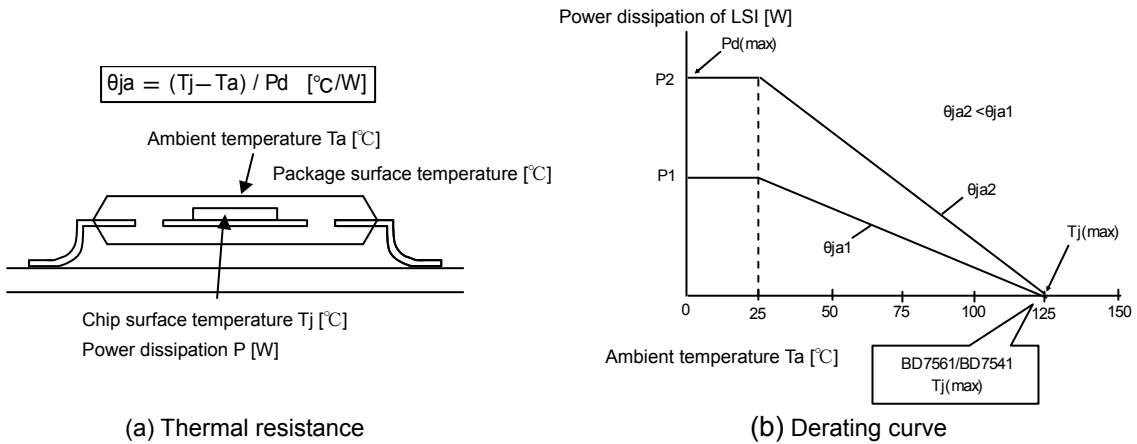
Fig.6 Thermal resistance and derating
