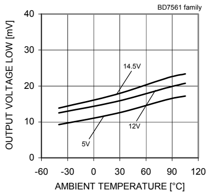
Fig.8 Output Voltage Low – Ambient Temperature ( R_L=10[k\Omega] )
