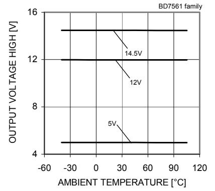
Fig.6 Output Voltage High – Ambient Temperature ( R_L=10[k\Omega] )
