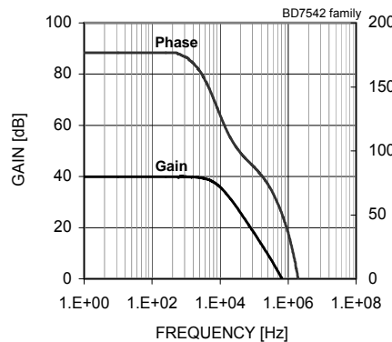
Fig. 23 Gain - Frequency
