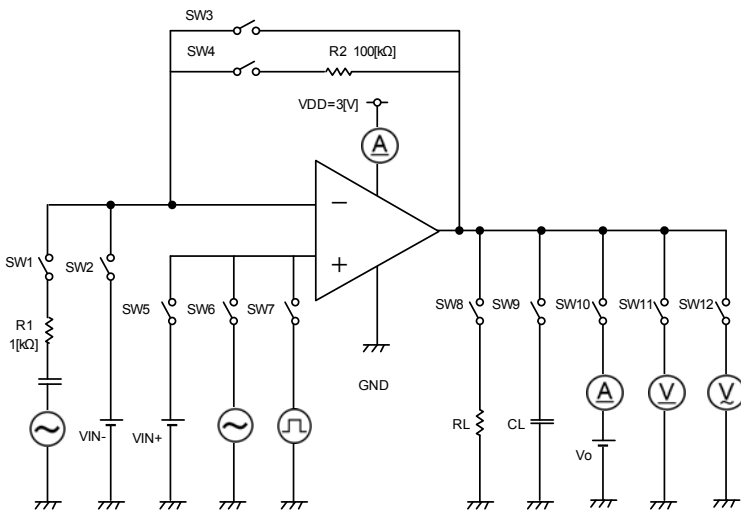
Fig3. Test circuit2
