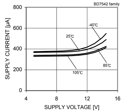
Fig.3 Supply Current - Supply Voltage
