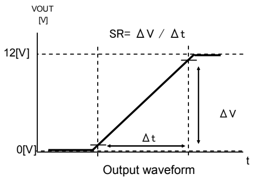
Fig4. Slew rate input output wave
