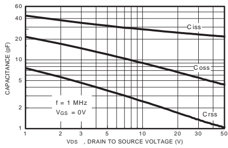
Figure 9. Capacitance Characteristics
