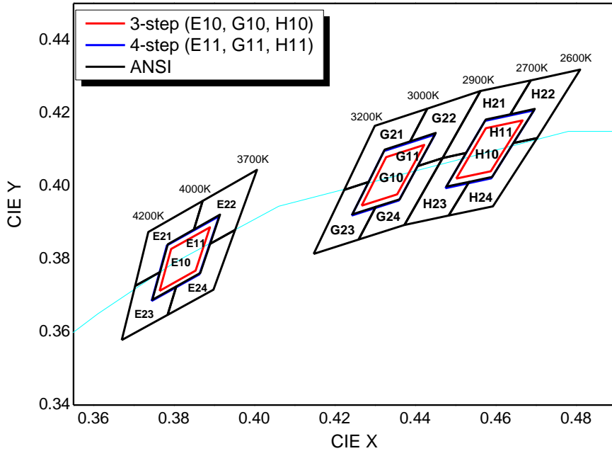
CIE Chromaticity Diagram (Warm white), Ta=25°C, IF=1000mA
