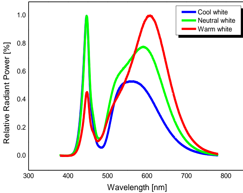
Fig 1. Color Spectrum, T_a = 25^\circ\text{C} , I_F = 1000\text{mA} , RH30\%
