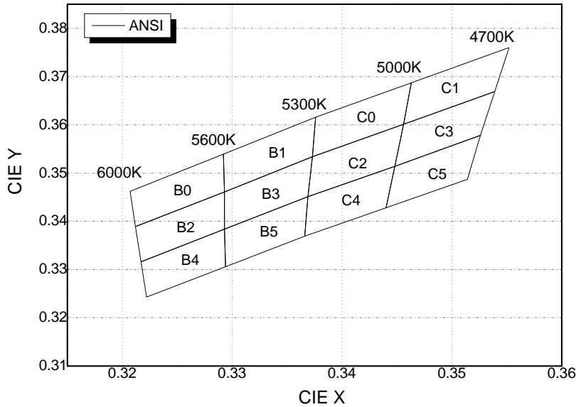
CIE Chromaticity Diagram (Cool white), Ta=25°C, IF=1000mA
