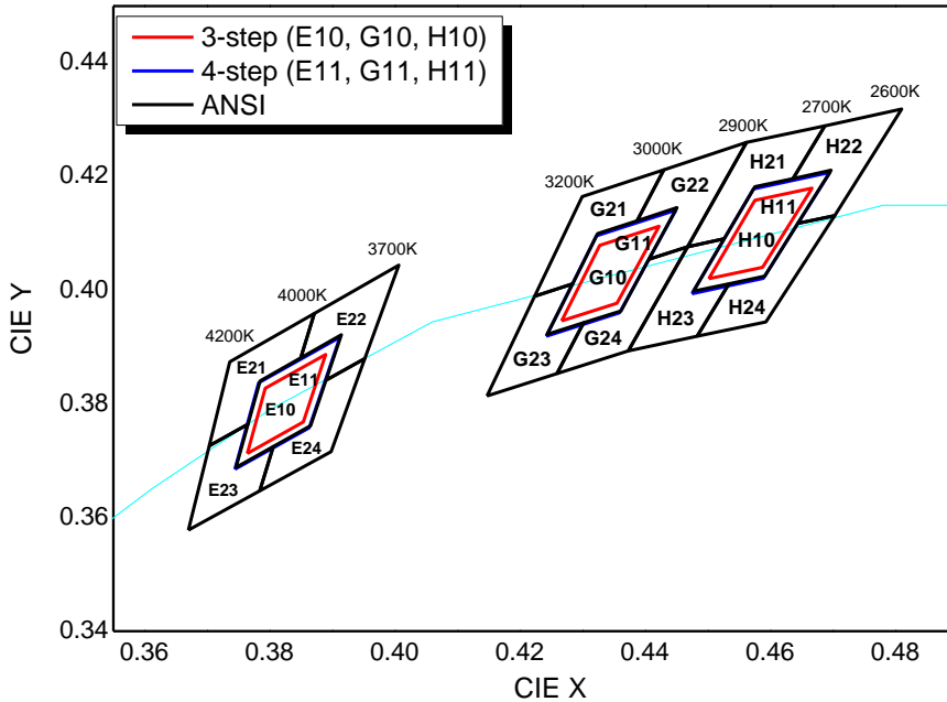
CIE Chromaticity Diagram (Warm white), Ta=25°C, IF=700mA
