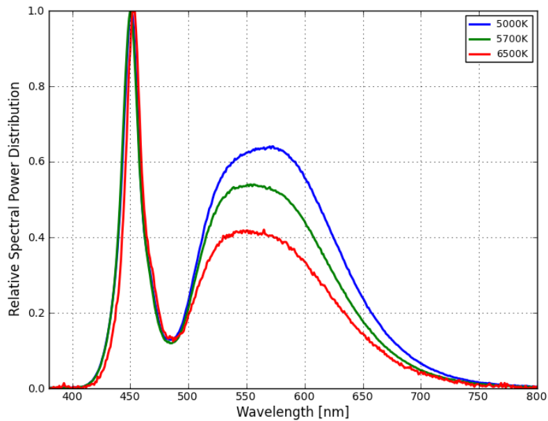
Figure 2. Emission color spectrum for MXZ7-PWxx
