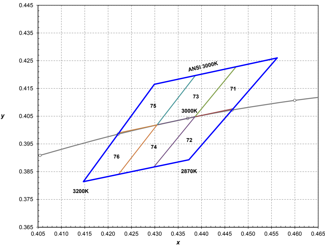
Figure 14. ANSI 3000K 1/6th color bin structure, forwards current = 30 mA, thermal pad temperature = 25°C.
