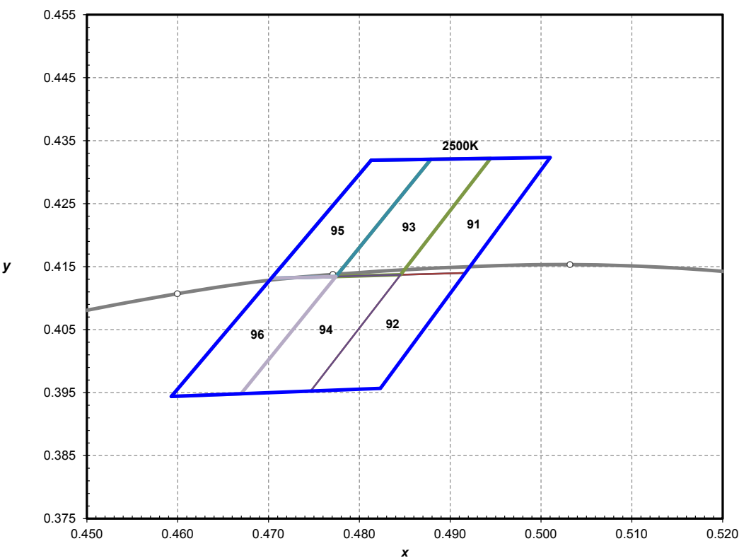
Figure 13. ANSI 2500K 1/6th color bin structure, forwards current = 30 mA, thermal pad temperature = 25°C.
