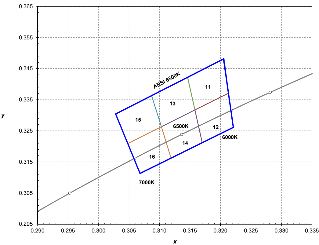
Figure 19. ANSI 6500K 1/6th color bin structure, forwards current = 30 mA, thermal pad temperature = 25°C.
