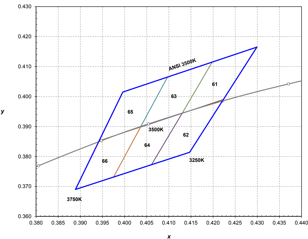
Figure 15. ANSI 3500K 1/6th color bin structure, forwards current = 30 mA, thermal pad temperature = 25°C.
