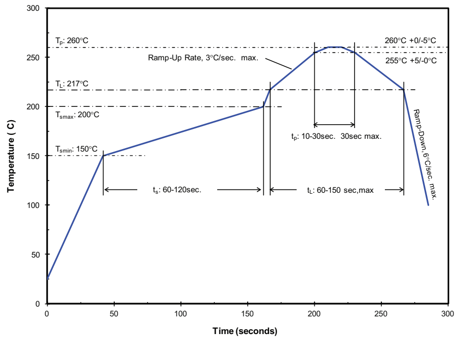
Temperature Profile for Table 5.
