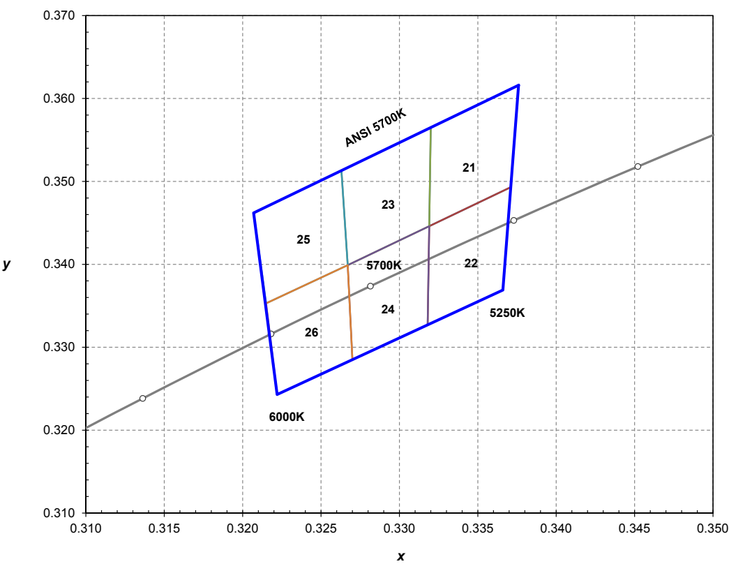
Figure 18. ANSI 5700K 1/6th color bin structure, forwards current = 30 mA, thermal pad temperature = 25°C.
