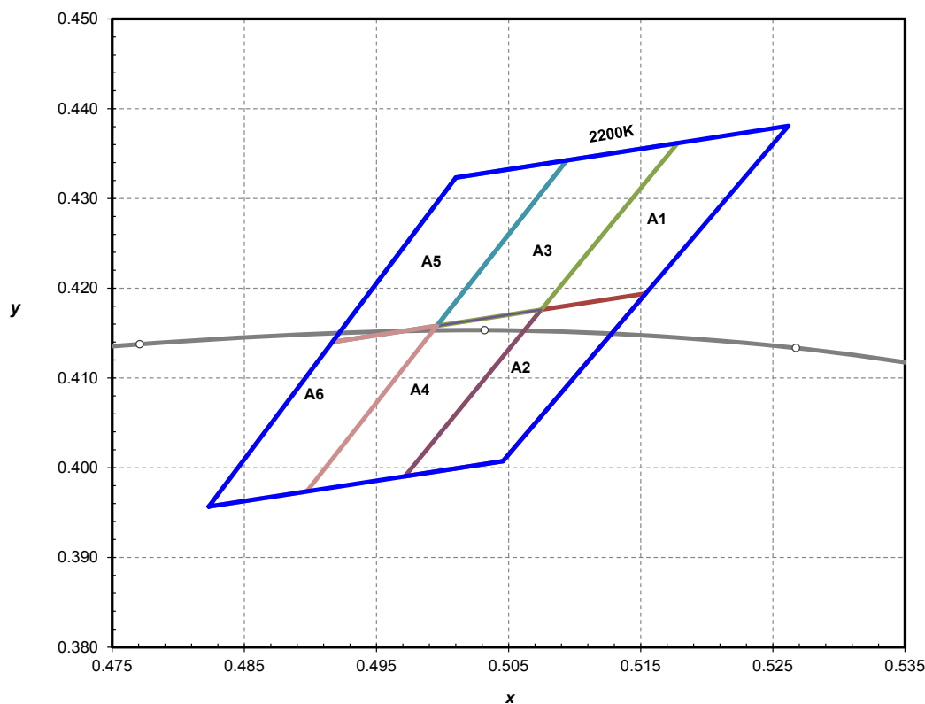
Figure 13. ANSI 2200K 1/6th color bin structure, forwards current = 30 mA, thermal pad temperature = 25°C.
