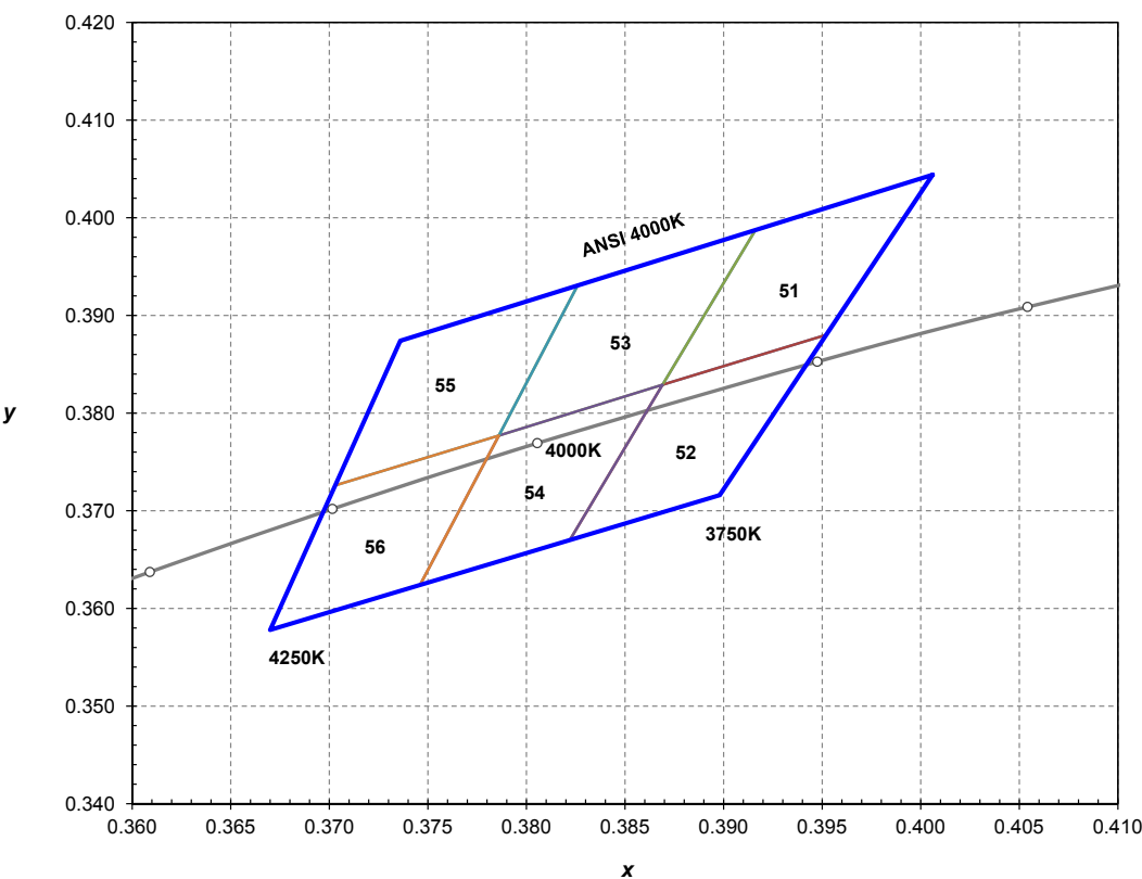
Figure 16. ANSI 4000K 1/6th color bin structure, forwards current = 30 mA, thermal pad temperature = 25°C.
