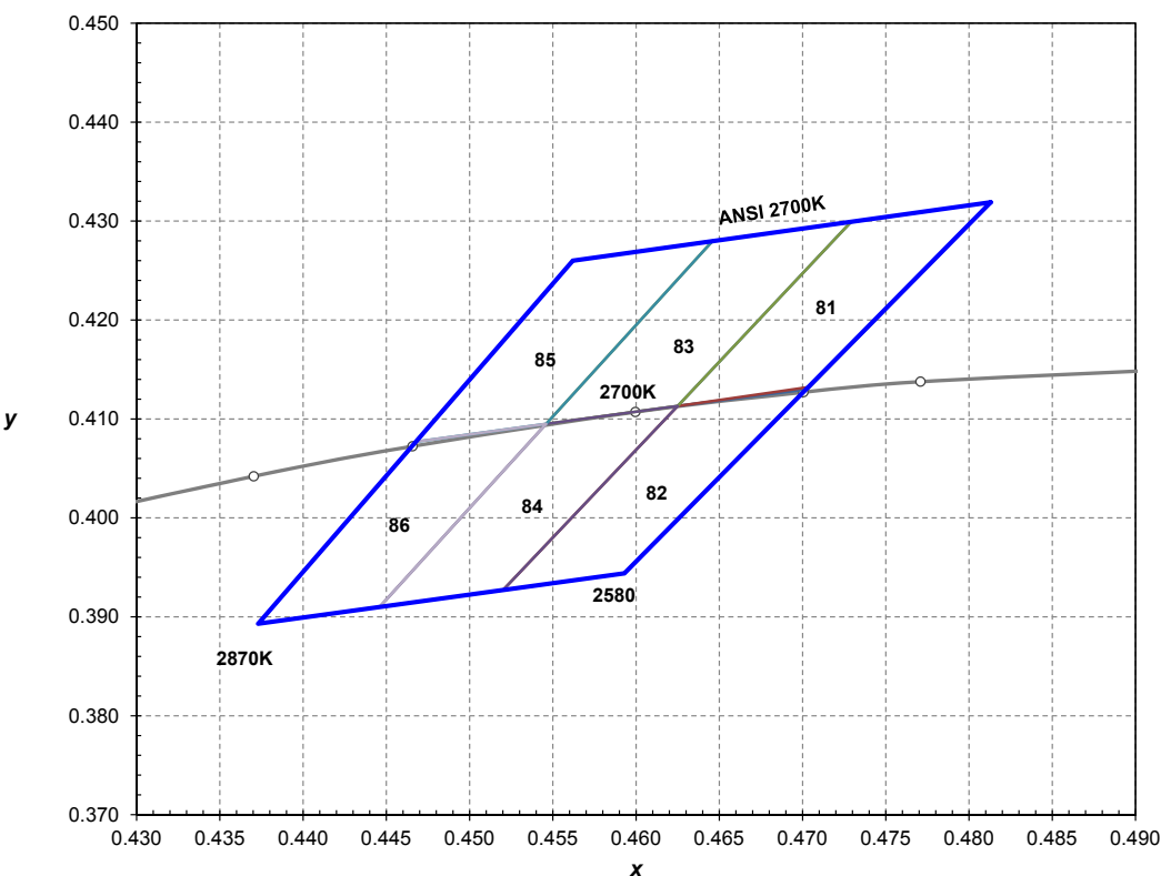
Figure 13. ANSI 2700K 1/6th color bin structure, forwards current = 30 mA, thermal pad temperature = 25°C.
