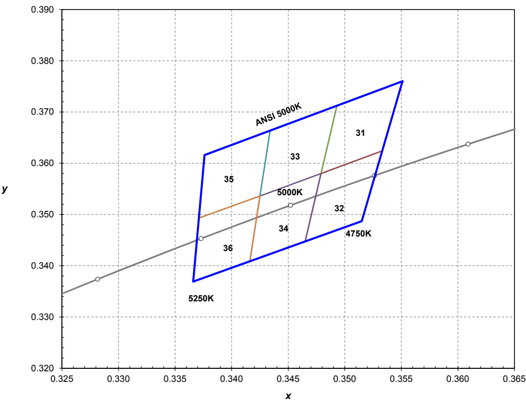
Figure 17. ANSI 5000K 1/6th color bin structure, forwards current = 30 mA, thermal pad temperature = 25°C.
