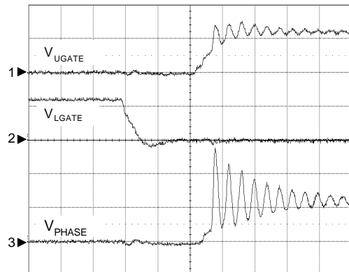
UGATE Rising
