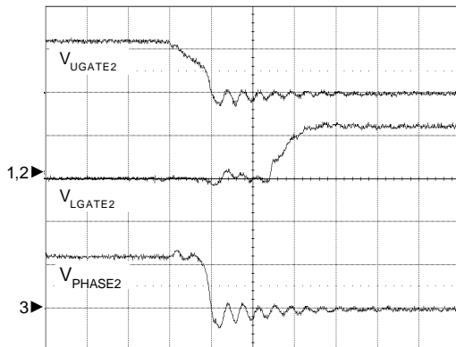
UGATE Falling
