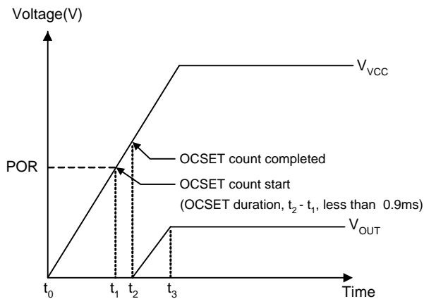
Figure 1. Soft-Start Interval
