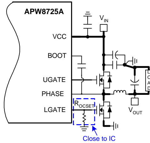
Figure 8. Layout Guidelines
