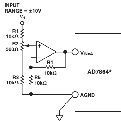
Figure 13. Full-Scale Adjust Circuit
