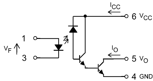
Fig. 5.1 Internal Circuit
