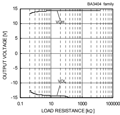
Maximum Output Voltage - Load Resistance (VCC/VEE=+15[V]/-15[V], Ta=25[°C])
