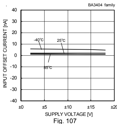
Input Offset Current - Supply Voltage (Vicm=0[V], VOUT=0[V])
