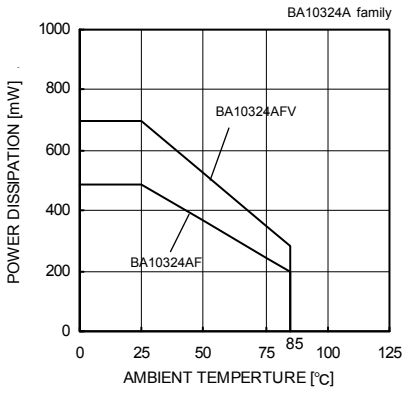
Fig. 25 Derating Curve
