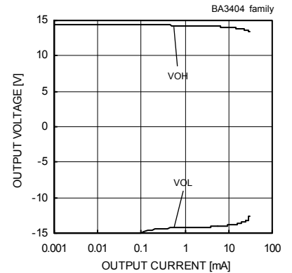
Output Voltage - Output Current (VCC/VEE=+15[V]/-15[V], Ta=25[°C])
