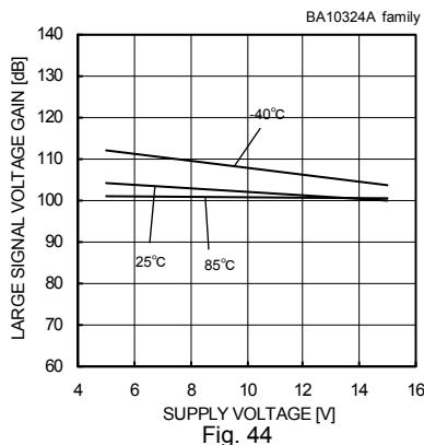
Large Signal Voltage Gain - Supply Voltage (RL=2[kΩ])
