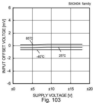
Input Offset Voltage - Supply voltage (Vicm=0[V], VOUT=0[V])
