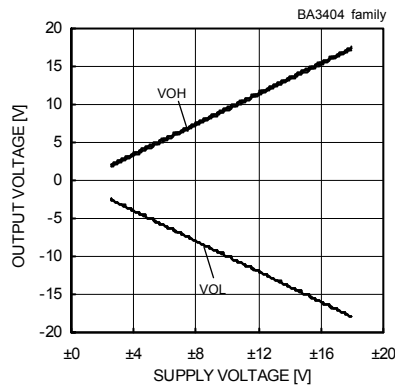
Maximum Output Voltage - Supply Voltage
