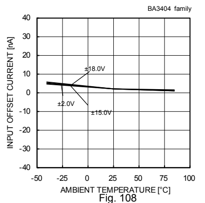
Input Offset Current - Ambient Temperature (Vicm=0[V], VOUT=0[V])
