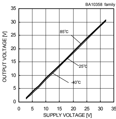
Fig. 4 Maximum Output Voltage - Supply Voltage ((RL=10[kΩ]))
