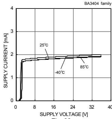
Supply Current - Supply Voltage
