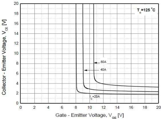
Saturation voltage vs. gate bias
