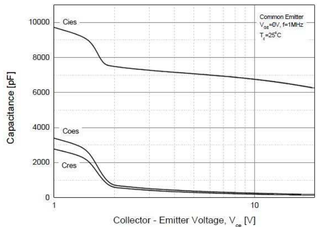
Capacitance characteristics
