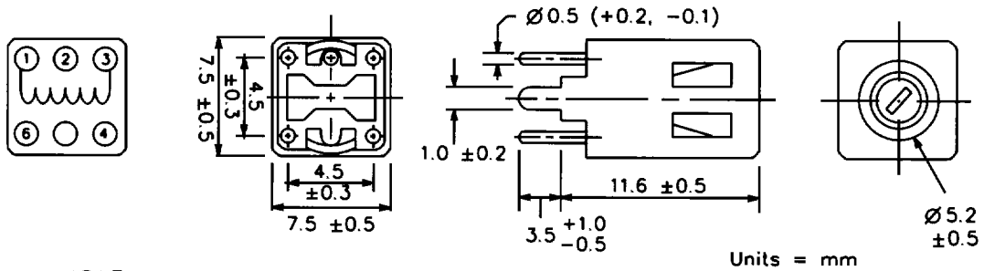
Style KS13XXN - with Plastic Sleeve
