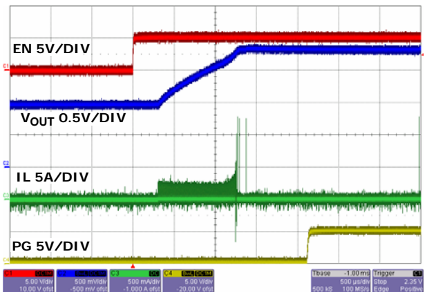
FIGURE 26. SOFT-START WITH PRE-BIASED V_{OUT}
