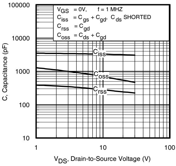
Fig 5. Typical Capacitance vs. Drain-to-Source Voltage www.irf.com
