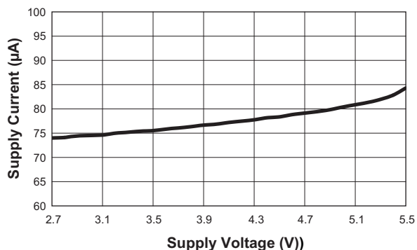
Supply Current vs. Supply Voltage (Switching)
