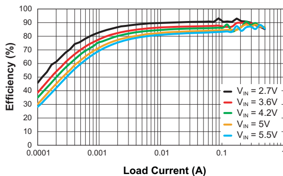
Efficiency vs. Load Current ( V_{OUT} = 1.8V )
