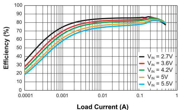
Efficiency vs. Load Current ( V_{OUT} = 1V )
