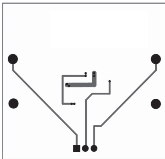
Figure 5: AAT1130 Evaluation Board Bottom Side PCB Layout.
