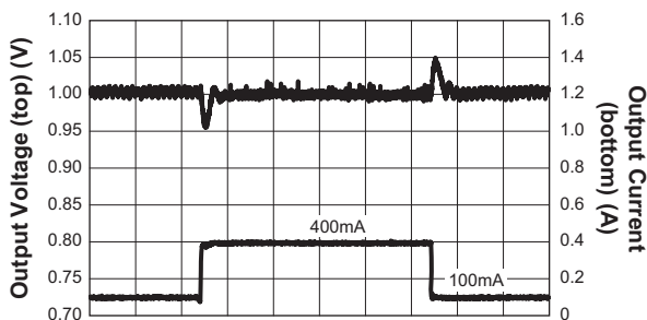
Load Transient (V_{OUT} = 1V; V_{IN} = 3.6V; C_{OUT} = 4.7\mu F; L = 1\mu H)
