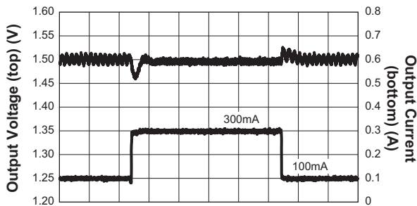
Load Transient (V_{OUT} = 1.5V; V_{IN} = 3.6V; C_{OUT} = 4.7\mu F; L = 1.5\mu H)
