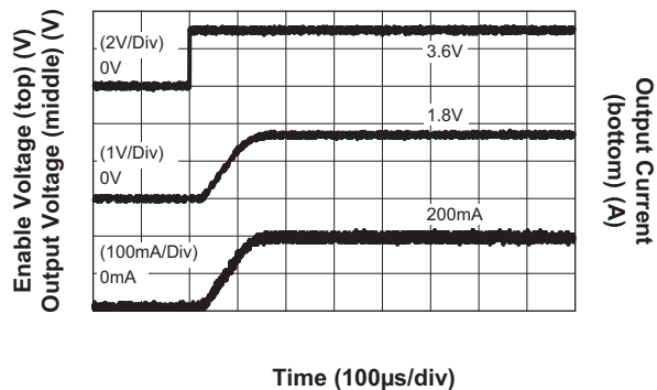
Soft-Start
