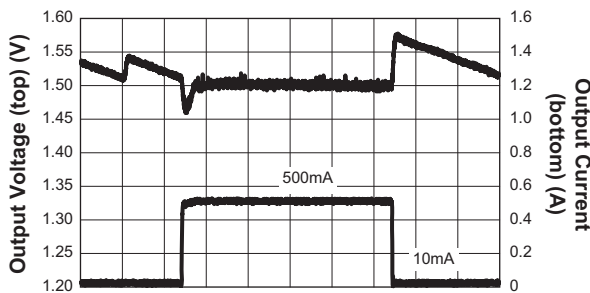
Load Transient (V_{OUT} = 1.5V; V_{IN} = 3.6V; C_{OUT} = 4.7\mu F; C_{FF} = 100pF; L = 1.5\mu H)
