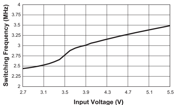
Switching Frequency vs. Input Voltage ( V_{OUT} = 1V ; C_{IN} = C_{OUT} = 2.2\mu F ; L = 1\mu H )
