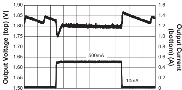
Load Transient (V_{OUT} = 1.8V; V_{IN} = 3.6V; C_{OUT} = 4.7\mu F; C_{FF} = 100pF; L = 1.5\mu H)
