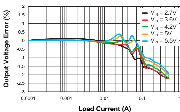
Output Voltage Error vs. Load Current ( V_{OUT} = 1V )
