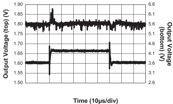
Line Transient
