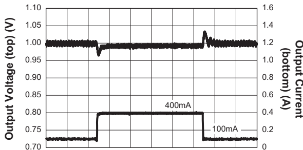
Load Transient (V_{OUT} = 1V; V_{IN} = 3.6V; C_{OUT} = 4.7\mu F; C_{FF} = 100pF; L = 1\mu H)
