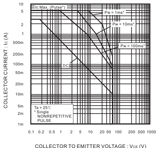
COLLECTOR TO EMITTER VOLTAGE : VCE (V) Safe Operating area
