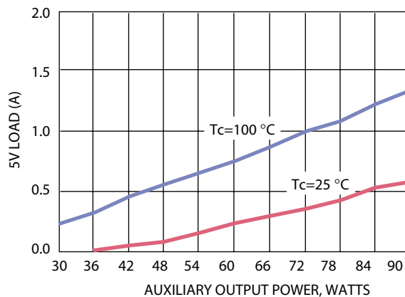
Minimum 5V Load vs. Auxiliary Output Power \mu V300 Triple Output Models
