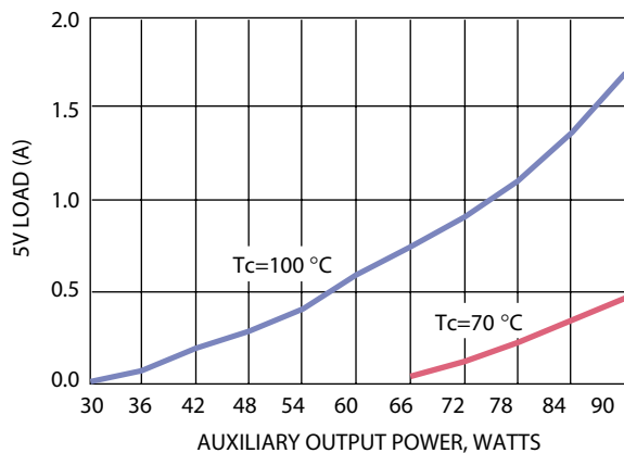
Minimum 5V Load vs. Auxiliary Output Power \mu V28 and \mu V48-Triple Output Models
