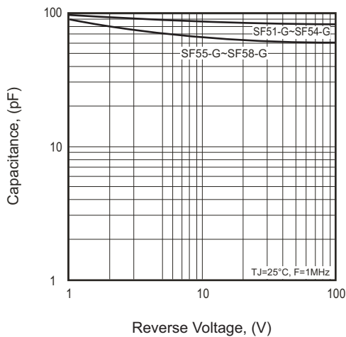
Fig.3-Typical Junction Capacitance
