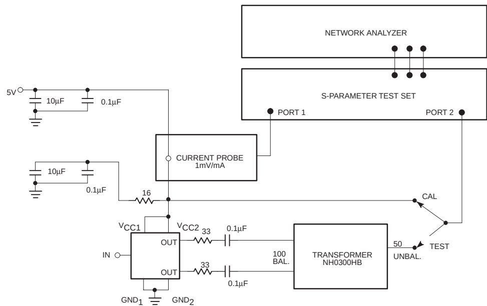
Test Circuit 3
