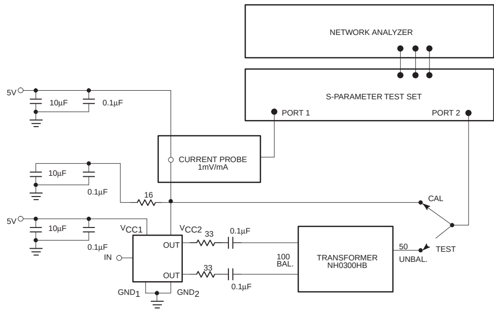
Test Circuit 5
