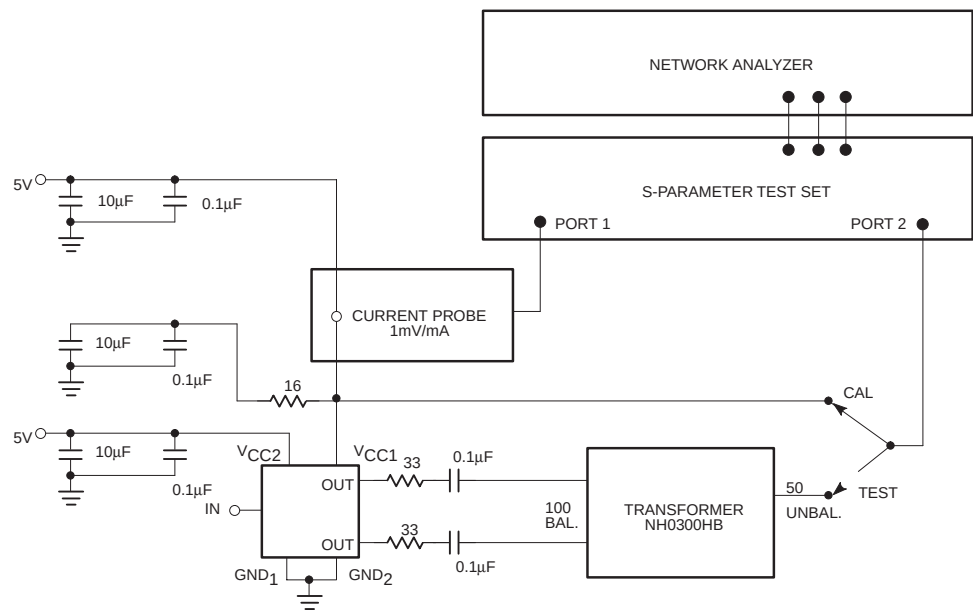
Test Circuit 4
