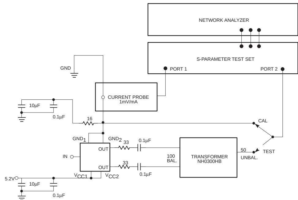
Test Circuit 6
