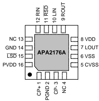
TQFN3x3-16 (Top View)
