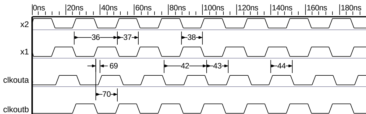
Figure 21. Clock—Active Mode
