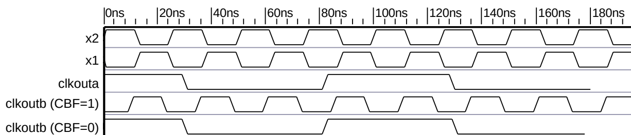
Figure 22. Clock—Power-Save Mode
