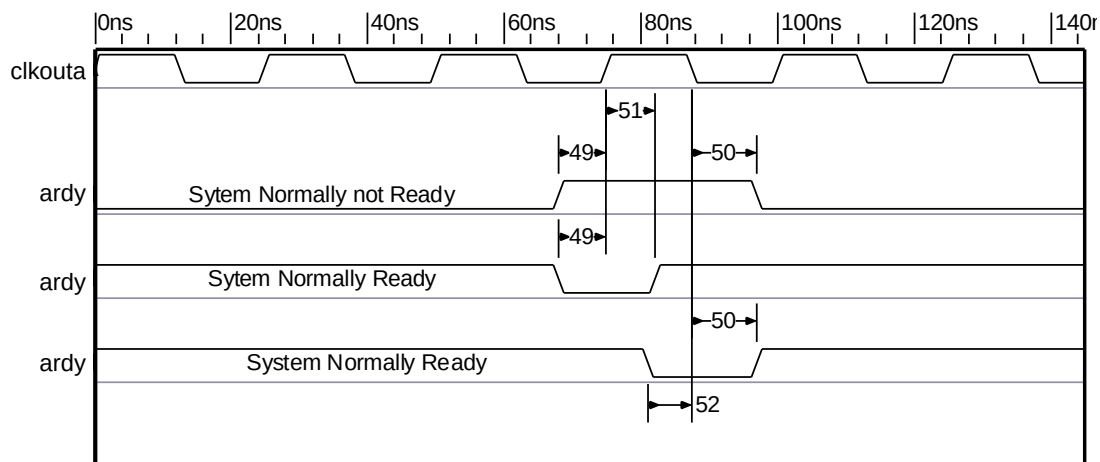
Figure 24. ardy—Asynchronous Ready
