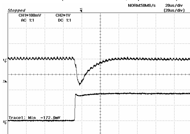
Figure 24: Typical transient response to step load change at 2.5A/\mu s from 50% to 100% of I_o , max at 3.3Vin, 2.5Vout (Cout = 1uF ceramic, 10uF tantalum)
