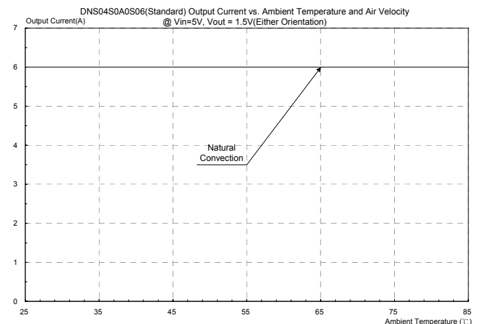
Figure 46: DNS04S0A0S06(Standard) Output current vs. ambient temperature and air velocity @ Vin=5V, Vout=1.5V(Either Orientation)
