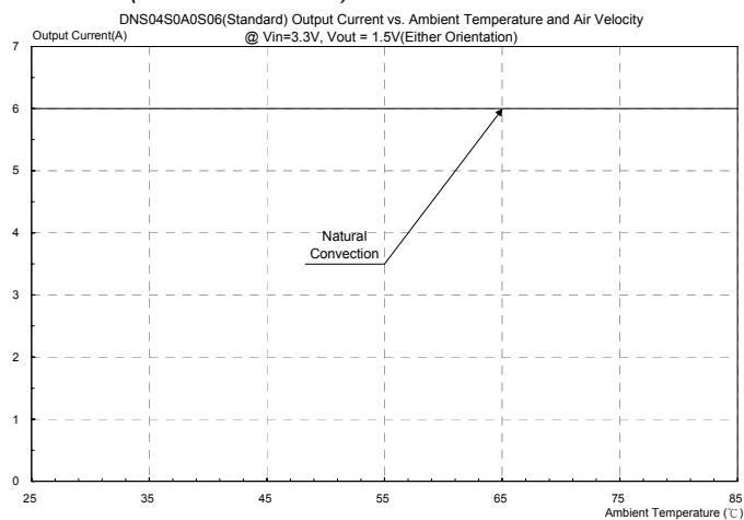
Figure 49: DNS04S0A0S06(Standard) Output current vs. ambient temperature and air velocity@Vin=3.3V, Vout=1.5V(Either Orientation)
