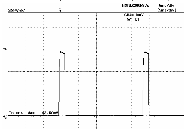
Figure 25: Typical transient response to step load change at 2.5A/\mu s from 100% to 50% of I_o , max at 3.3Vin, 1.8Vout (Cout = 1uF ceramic, 10uF tantalum)
