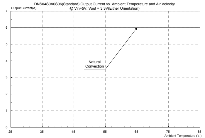
Figure 45: DNS04S0A0S06(Standard) Output current vs. ambient temperature and air velocity @ Vin=5V, Vout=3.3V(Either Orientation)
