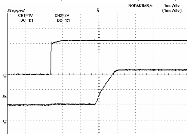
Figure 26: Typical transient response to step load change at 2.5A/\mu s from 50% to 100% of I_o , max at 3.3Vin, 1.8Vout (Cout = 1uF ceramic, 10uF tantalum)
