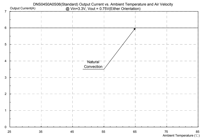
Figure 50: DNS04S0A0S06(Standard) Output current vs. ambient temperature and air velocity@Vin=3.3V, Vout=0.75V(Either Orientation)
