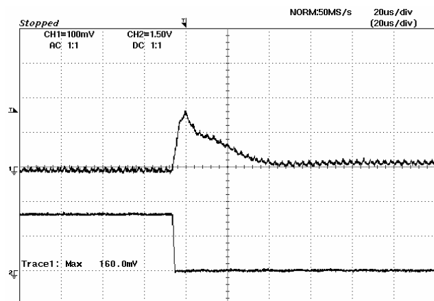
Figure 23: Typical transient response to step load change at 2.5A/\mu s from 100% to 50% of I_o , max at 3.3Vin, 2.5Vout (Cout = 1uF ceramic, 10uF tantalum)
