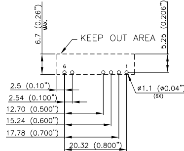
RECOMMENDED PWB PAD LAYOUT
