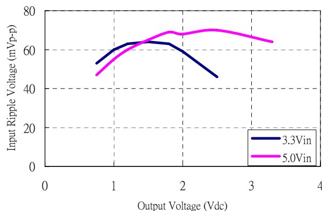
Figure 33: Input voltage ripple for various output models, I_o = 6A ( C_{IN} = 4 \times 100\mu F tantalum // 2x47 \mu F ceramic)
