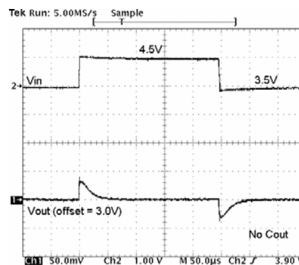
Figure 16. 3.5V - 4.5V Line Step ( t_r=1\mu s , No C_{OUT} )
