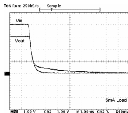
Figure 24. Power-Down ( I_{LOAD}=5mA )
