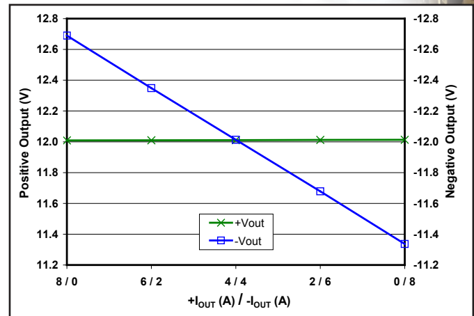
Figure 8: Load regulation vs. load current with power fixed at 80% load (96W) and load currents split as shown between the +12V and -12V outputs, at nominal input voltage and TCASE = 25°C.
