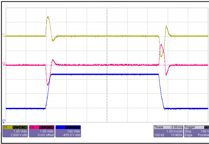
Figure 19: Output voltage response to step-change in input voltage (155V - 400V - 155V). Load cap: 10 \mu F, 100 mW ESR tantalum cap and 1 \mu F ceramic cap. Ch 1: +Vout (1V/div); Ch 2: -Vout (1V/div); Ch 3: Vin (100V/div).
