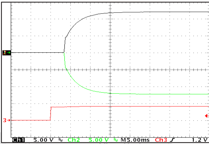
Figure 13: Turn-on transient at full rated load current (resistive load) (5 ms/div). Input voltage pre-applied. Ch 1: +Vout (5V/div); Ch 2: -Vout (5V/div); Ch 3: Enable1 input (5V/div).
