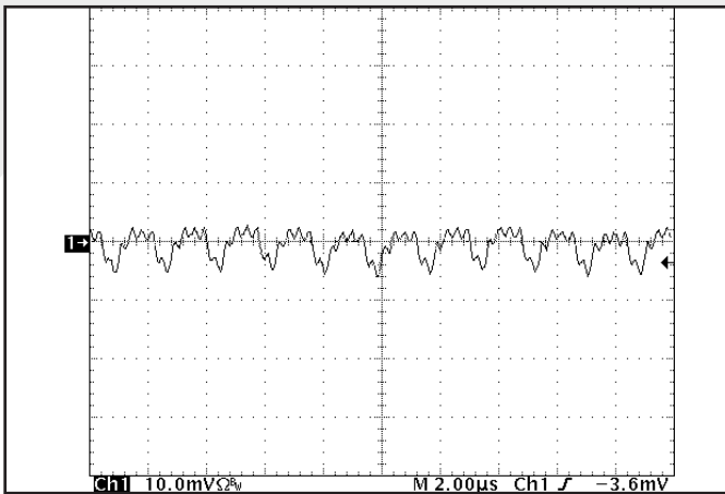
Figure 21: Input terminal current ripple, i_c , at full rated output current and nominal input voltage with SynQor MQ filter module (100 mA/div). Bandwidth: 20MHz. See Fig 20.
