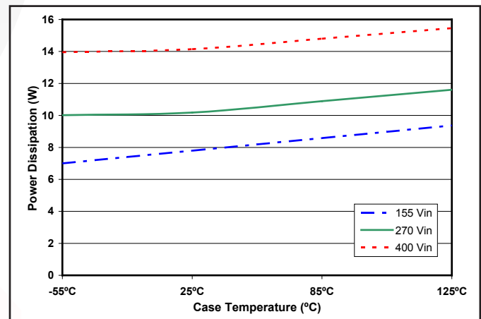
Figure 6: Power dissipation at 60% load (3A load on +12V and 3A load on -12V) versus case temperature for V_{in} = 155V, 270V, and 400V .
