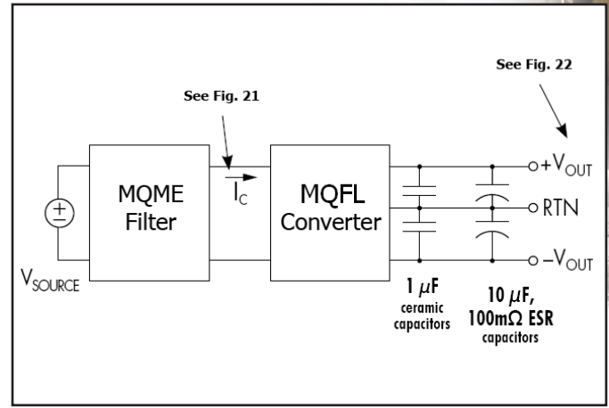
Figure 20: Test set-up diagram showing measurement points for Input Terminal Ripple Current (Fig 21) and Output Voltage Ripple (Fig 22).
