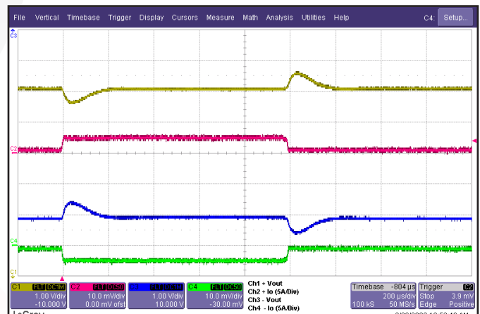
Figure 18: Output voltage response to step-change in total load current (10%-50%-10%) of total Iout (max) split 50%/50%. Load cap: 1 \mu F ceramic cap and 10 \mu F, 100 mW ESR tantalum cap. Ch 1: +Vout (1 V/div); Ch 2: +Iout (5A/div); Ch 3: -Vout (1 V/div); Ch 4: -Iout (5A/div).
