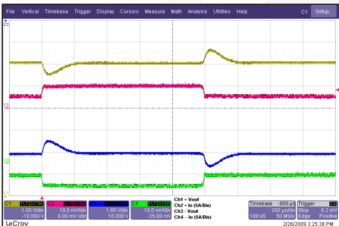
Figure 17: Output voltage response to step-change in total load current (50%-100%-50%) of total Iout (max) split 50%/50%. Load cap: 1 \mu F ceramic cap and 10 \mu F, 100mW ESR tantalum cap. Ch 1: +Vout (1 V/div); Ch 2: +Iout (5A/div); Ch 3: -Vout (1 V/div); Ch 4: -Iout (5A/div).
