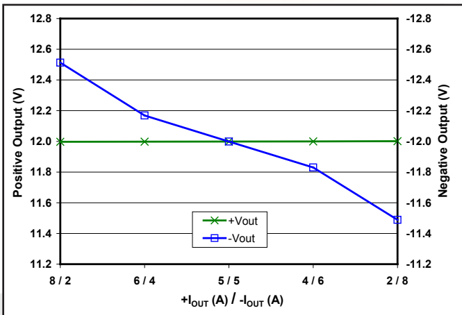
Figure 7: Load regulation vs. load current with power fixed at full load (120W) and load currents split as shown between the +12V and -12V outputs, at nominal input voltage and TCASE = 25°C.
