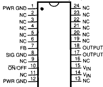
24-LEAD SOIC (WM)
