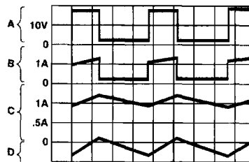
Switching Waveforms
