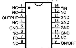
16-LEAD DIP (N)
