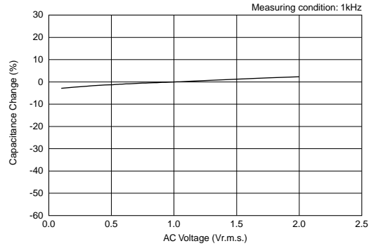
High Dielectric Constant Type: GRM155R71E103KA01
