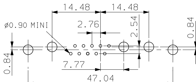
LAYOUT DIMENSIONS (after plating) CONNECTOR SIDE VIEW
