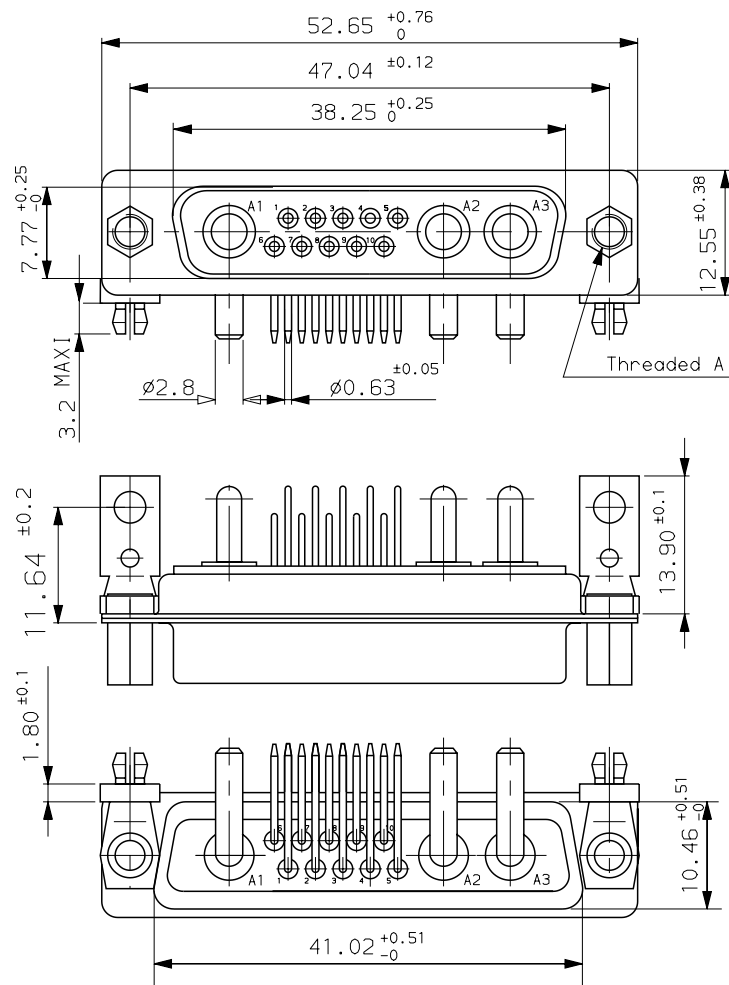
LAYOUT DIMENSIONS (after plating) CONNECTOR SIDE VIEW
