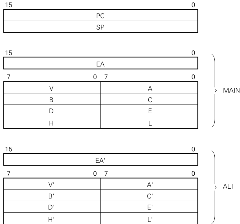
Fig. 2-1 Register Configuration
