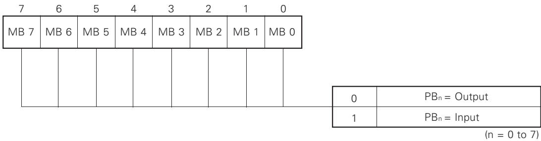
Fig. 2-9 Mode B Register Format
