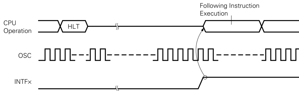
Fig. 4-3 HALT Mode Release Timing (in DI State)
