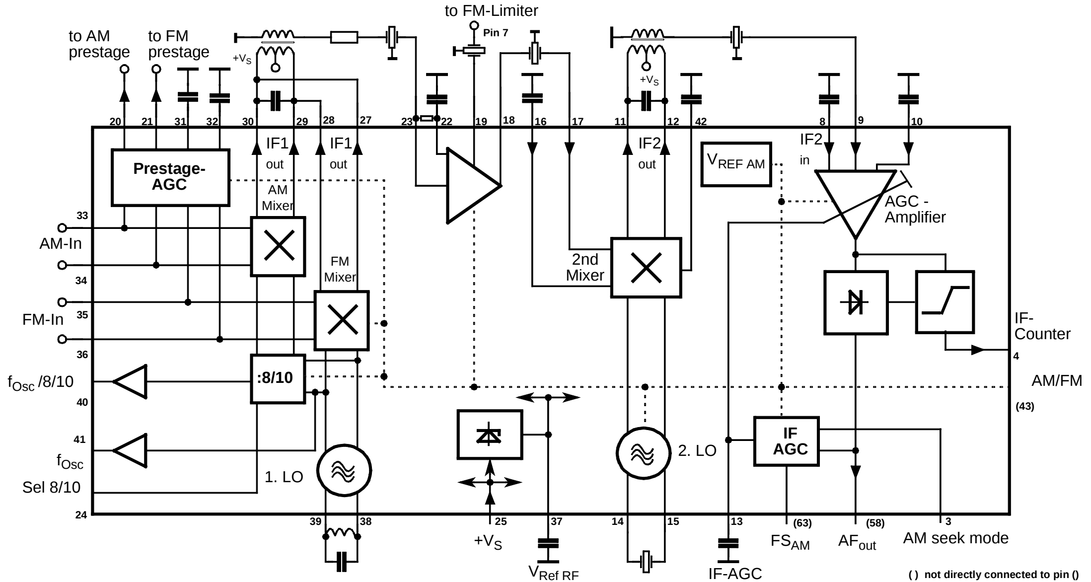
Block Diagram AM/FM Receiver
