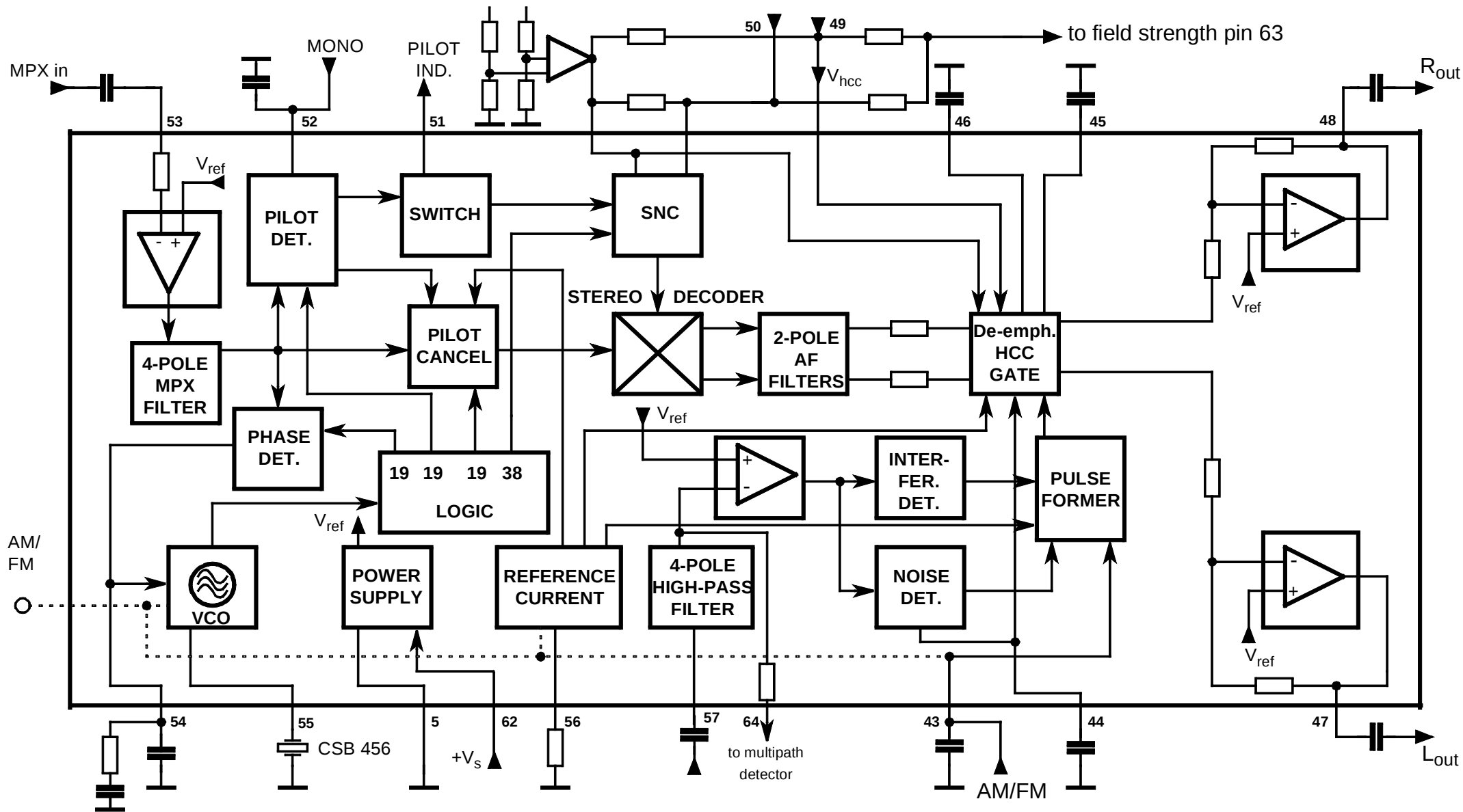
Block Diagram Stereodecoder/Noiseblanker
