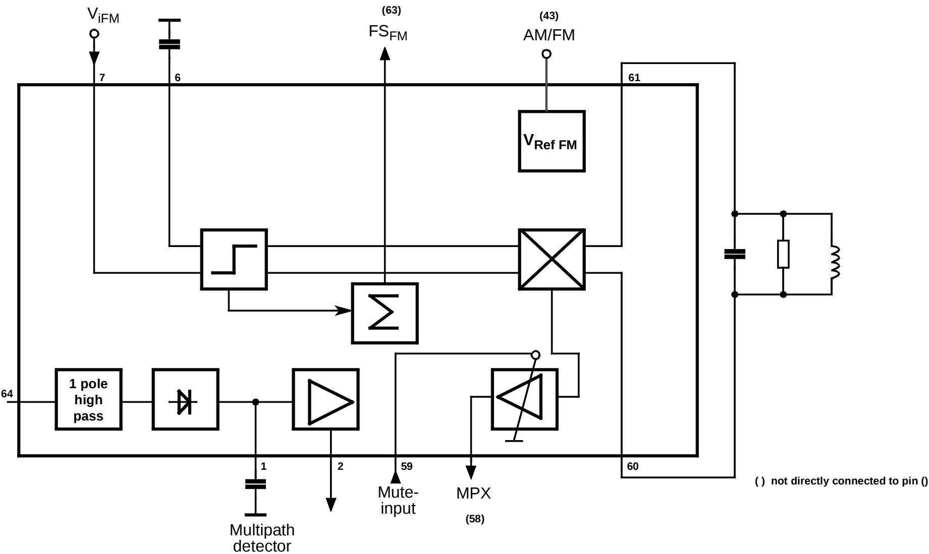
Block Diagram FM-IF Amplifier
