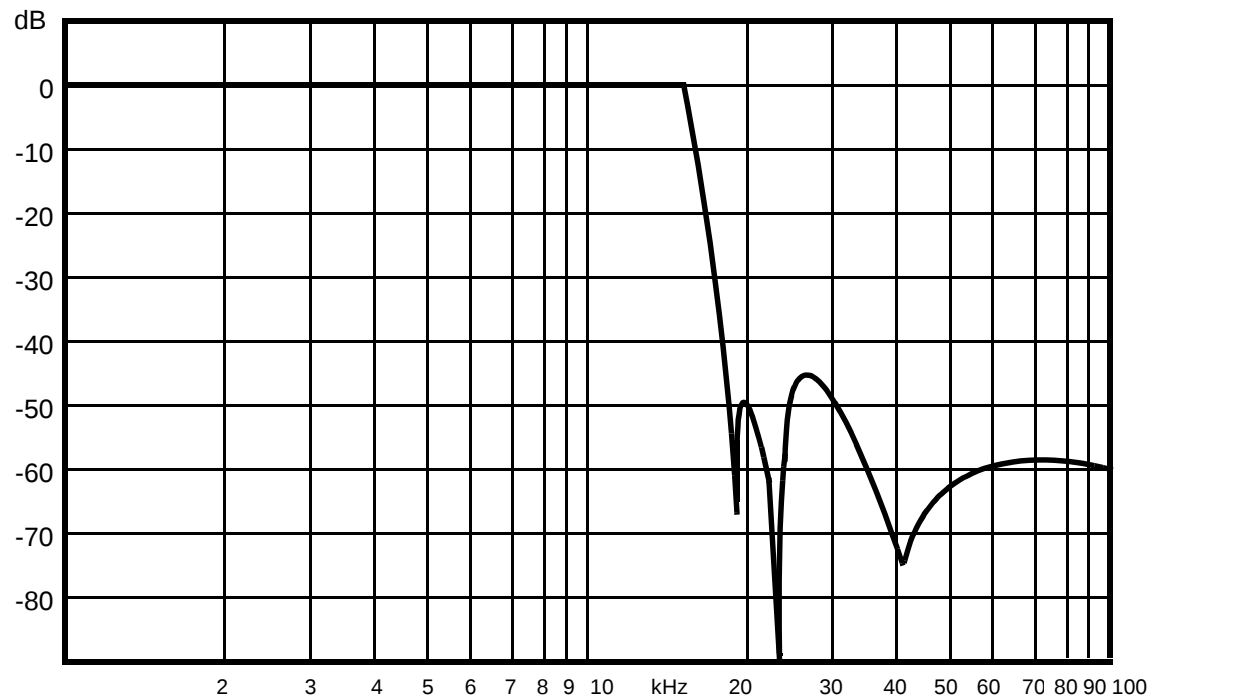
Low pass filter with 19 kHz Notch
