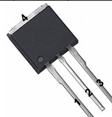
T0262 Standard Metal Heatsink 1=Gate, 2&4=Drain, 3=Source.
