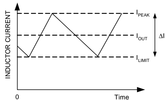
Figure 1. Current-Limit Algorithm
