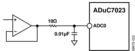
Figure 28. Buffering Single-Ended/Pseudo Differential Input
