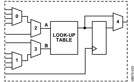
Figure 39. PLA Element
