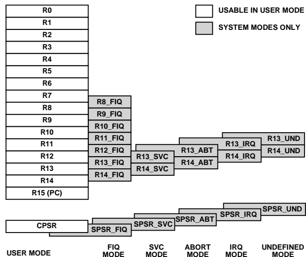
Figure 14. Register Organization
