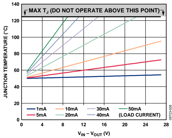
Figure 23. 500 mm 2 of PCB Copper, T A = 50°C
