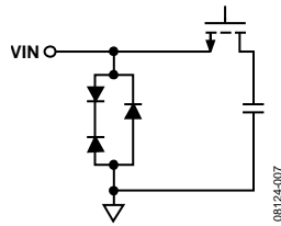
Figure 55. Equivalent Analog Input Circuit
